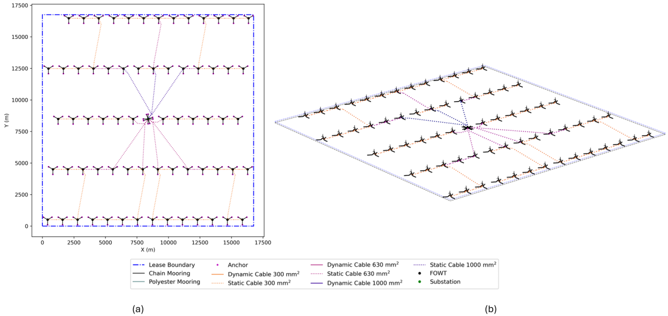
Figure 24. Gulf of America array layout and cable routing in (a) plan view and (b) 3 dimensions
