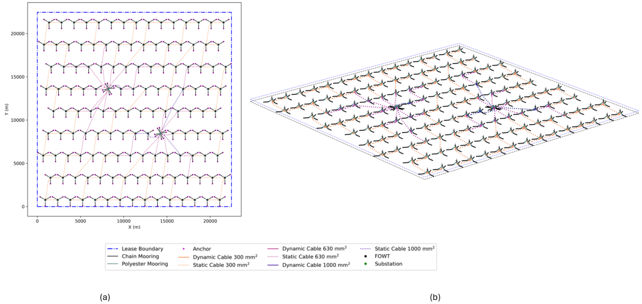
Figure 18. Gulf of Maine array layout and cable routing in (a) plan view and (b) 3 dimensions
