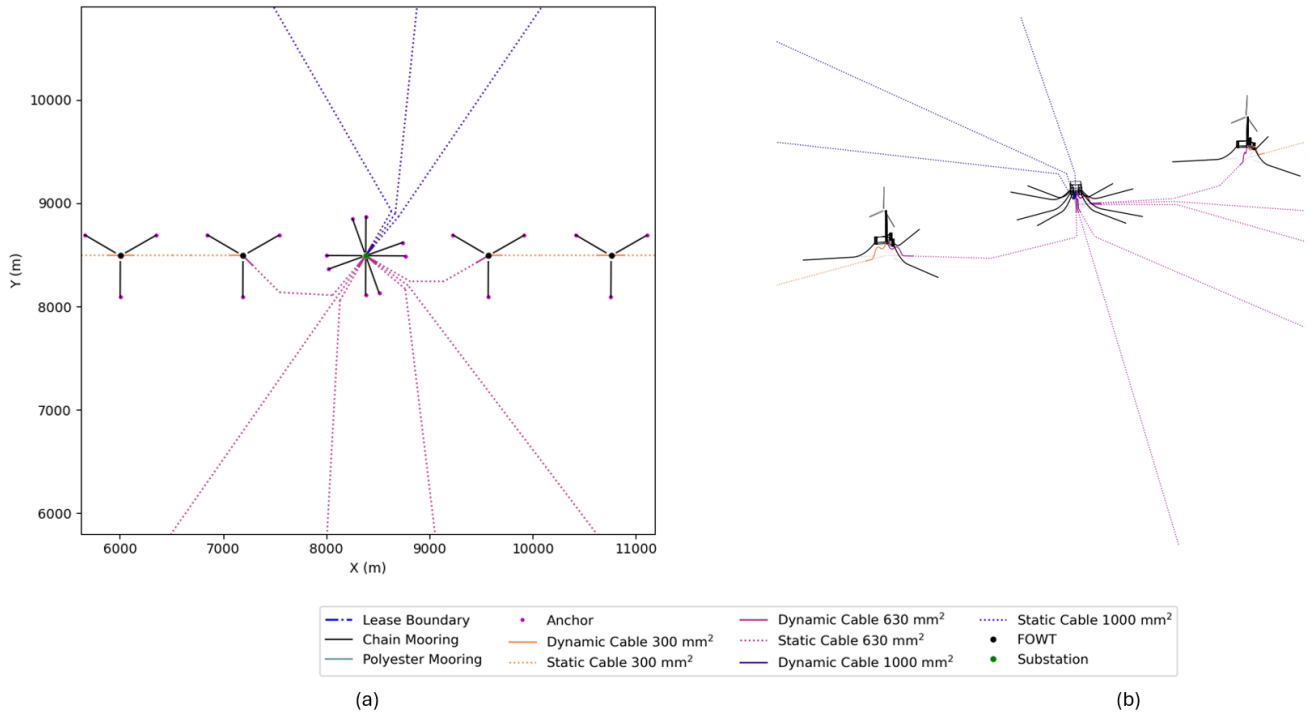
Figure 25. Final routing of intra-array cables into substation for the Gulf of America array in (a) plan view and (b) 3 dimensions
