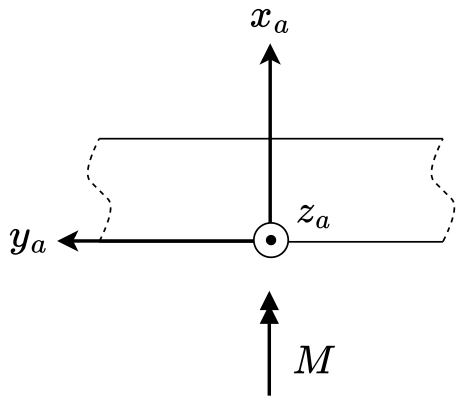
Figure 1. Original Amiet's coordinate system.
