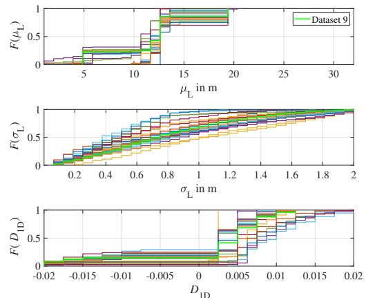
Figure 10. Resulting CDFs of the deterministic model-updating procedures for combination I-III based on the modal parameters of all datasets. The results for dataset 9 are highlighted in green.
