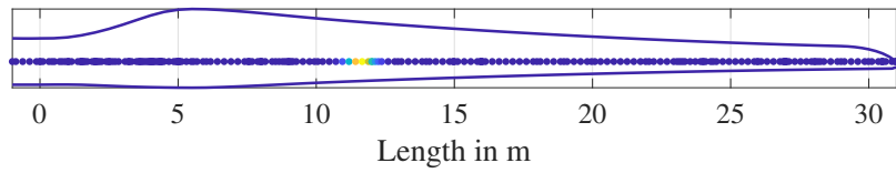
Figure 12. Visualization of the stiffness reduction based on x_{ID,optimal} , denoted by red crosses in Figure 11, in the beam model. The schematic rotor blade geometry is additionally outlined.
