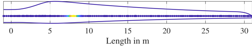
Figure 13. Visualization of the correct stiffness reduction in the beam model. The schematic rotor blade geometry is additionally outlined.
