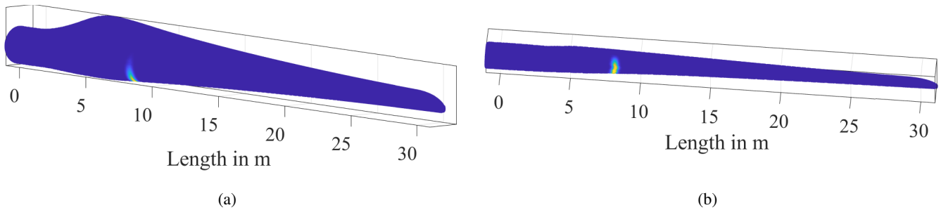
Figure 17. Visualization of the correct stiffness reduction in the shell model. View of the (a) pressure side and (b) leading edge.
