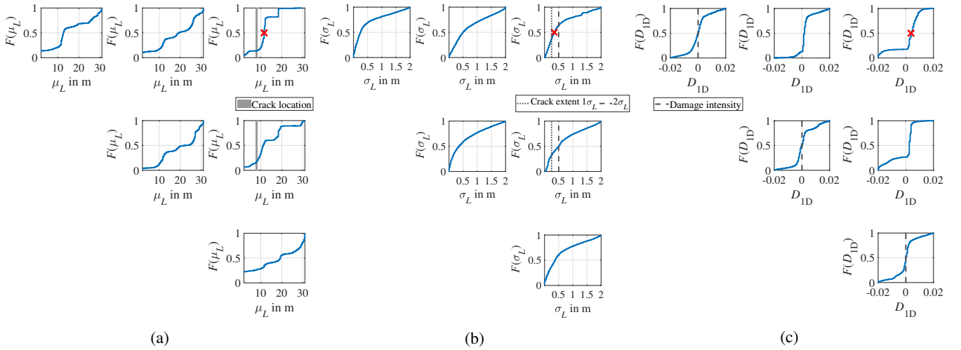
Figure 11. Resulting CDFs of the SDMU approach applied to the beam model using the one-dimensional damage distribution function parameterized by the three design variables (a) \mu_L , (b) \sigma_L and (c) D_{1D} , with settings given in Table 8. The red crosses added for combination I-III indicate an example optimal design variable vector.
