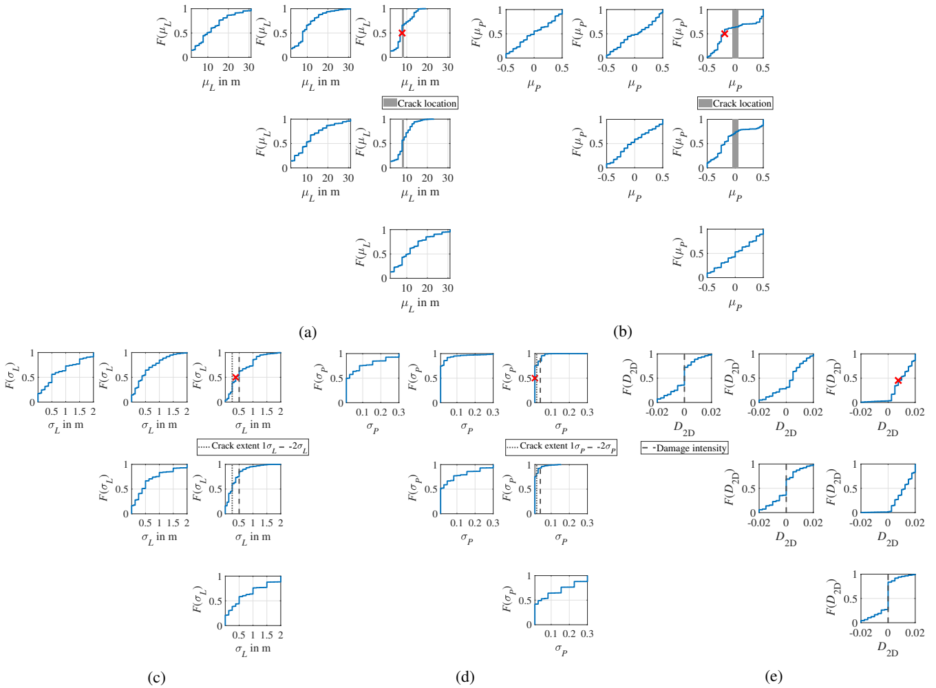
Figure 15. Resulting CDFs of the SDMU approach applied to the shell model using the two-dimensional damage distribution function parameterized by the five design variables (a) \mu_L , (b) \mu_P , (c) \sigma_L , (d) \sigma_P and (e) D_{2D} . The red crosses added for combination I-III indicate an example optimal design variable vector.
