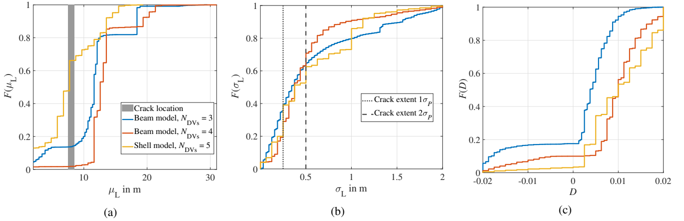
Figure 18. Resulting CDFs of the SDMU procedure for combination I-III – comparison of all three parameterizations of the damage distribution function. Design variables (a) \mu_L , (b) \sigma_L and (c) D .
