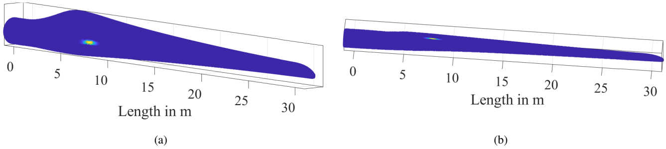
Figure 16. Visualization of the stiffness reduction based on \alpha_{2D, optimal} , denoted by red crosses in Figure 15, in the shell model. View of the (a) pressure side and (b) leading edge.
