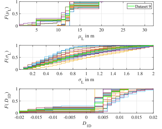
Figure 10. Resulting CDFs of the deterministic model-updating procedures for combination I-III based on the modal parameters of all datasets. The results for dataset 9 are highlighted in green.
