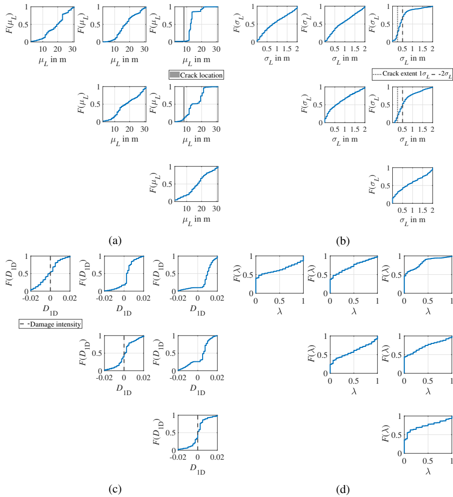
Figure 14. Resulting CDFs of the SDMU approach applied to the beam model using the one-dimensional damage distribution function parameterized by the four design variables (a) \mu_L , (b) \sigma_L , (c) D_{1D} and (d) \lambda , with settings given in Table 8.
