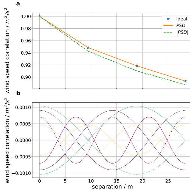
Figure 4. Negative DFT coefficients contribution. Fig4a: the theoretical correlation function in blue stars, the correlation function computed using Eq. (8) assuming negative values in the PSD in the PSD in orange, the correlation function computed using the absolute value of the PSD in dashed green. Fig4b: the different colors represent the contribution to the correlation function computation of different DFT coefficients. The contribution of the negative coefficients is represented by continuous lines, the contribution of the same coefficients but with a positive value in dashed lines. The difference between the sum of the two sets of lines gives the expected error in using the absolute value of the PSD.
