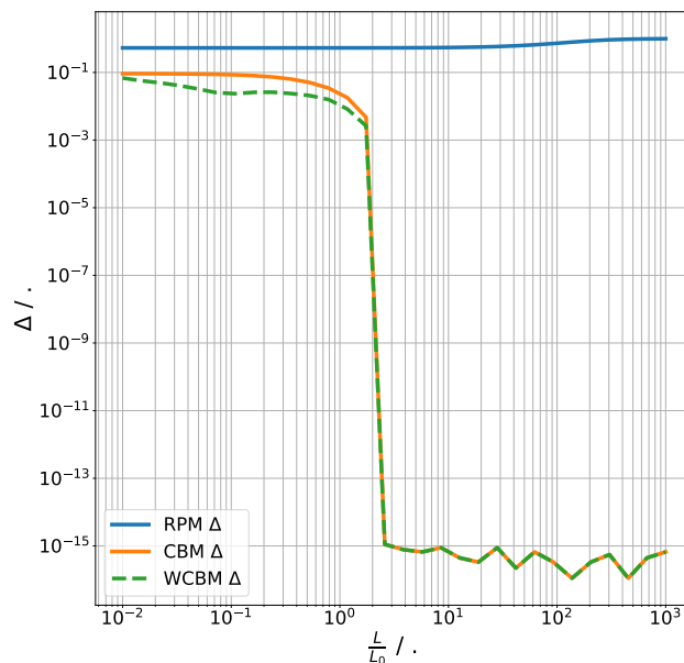
Figure 5. (Increased the spatial domains) Methods comparison. RPM error in blue, CBM error in orange, WCBM in dashed green. The x axis indicates the ratio between the considered spatial domain and the turbulence outer scale.
