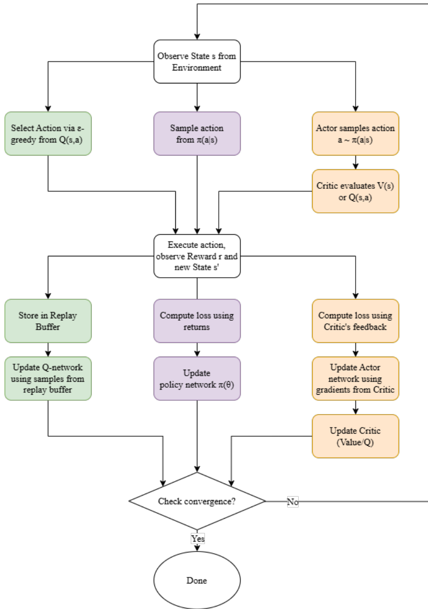
Figure 2. Overview of single-agent DRL-Deep Reinforcement Learning algorithm families
