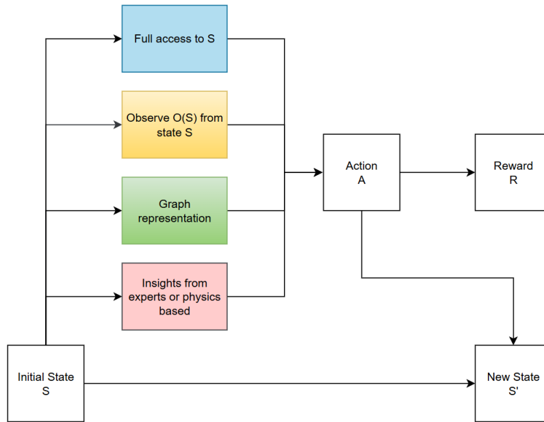
Figure 5. Overview of problem formulations in DRL-Deep Reinforcement Learning models: MDP-Markov Decision Problem (blue), PO-MDP-Partially Observable Markov Decision Problem (yellow), graph/network-based formulation (green), and hierarchical approaches (pink)
