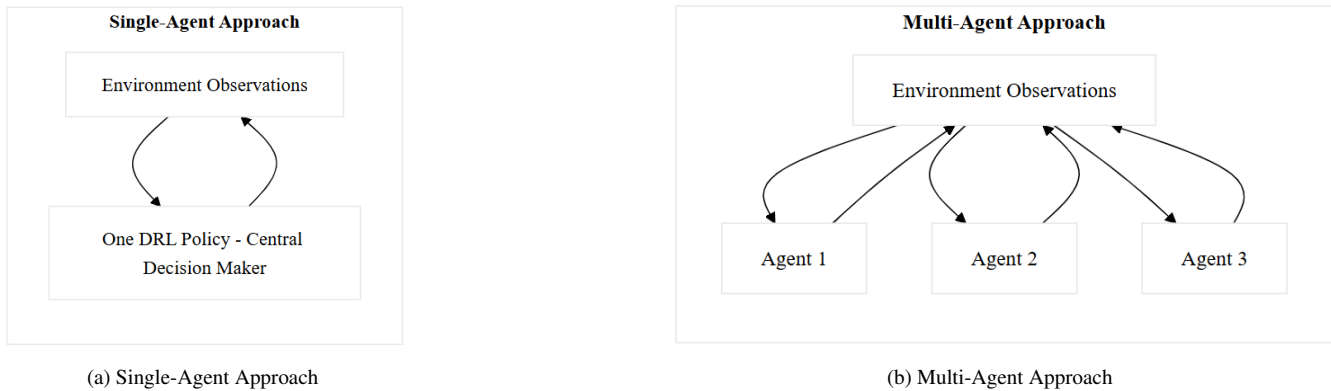
Figure 3. Comparison of Single-Agent and Multi-Agent DRL Deep Reinforcement Learning Approaches
