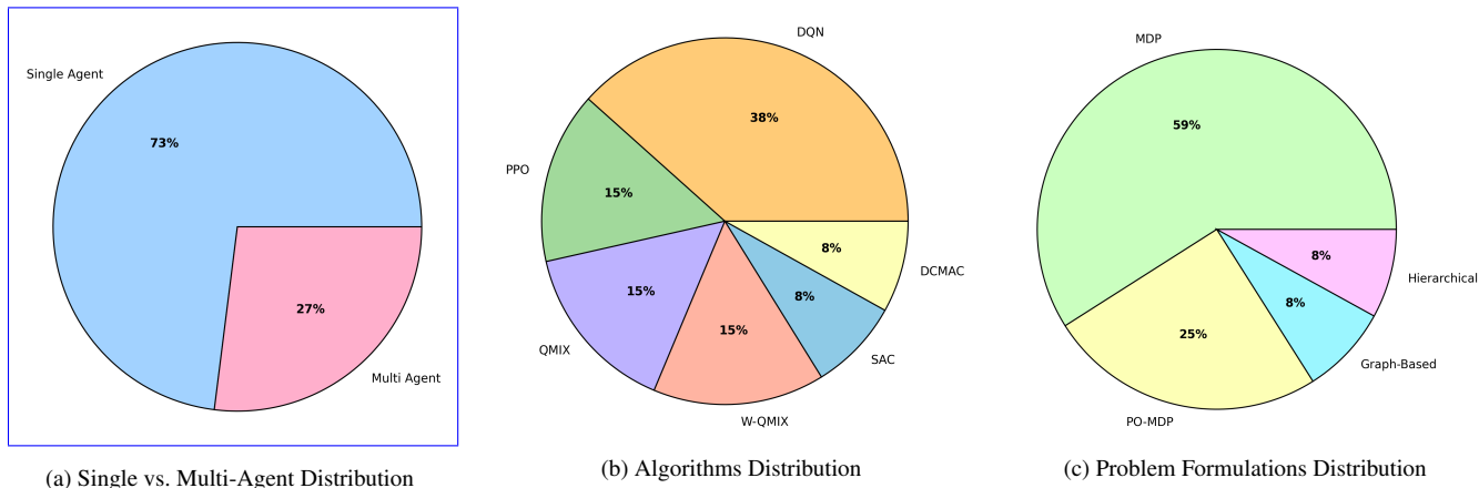
Figure 7. Comparative view of single vs. multi-agent methods, main Deep Reinforcement Learning algorithms, and problem formulations in the reviewed literature.
