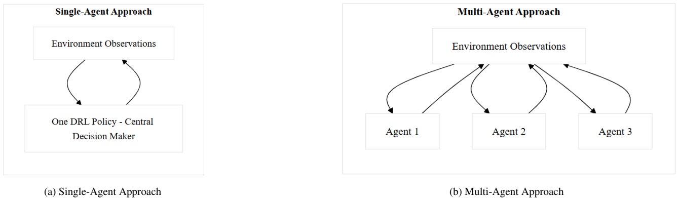
Figure 3. Comparison of Single-Agent and Multi-Agent Deep Reinforcement Learning Approaches
