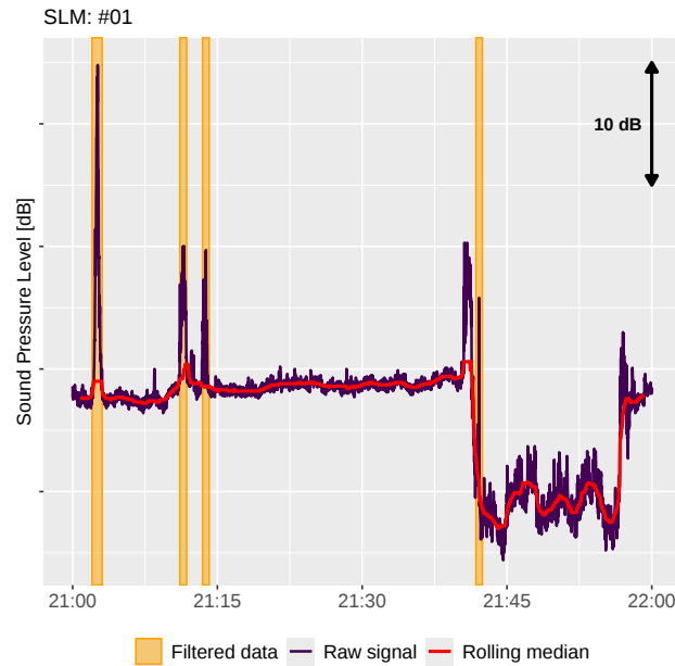
Figure 10. An example of automatic outlier detection for SLM #01. The rolling median is calculated from the raw signal and periods of \pm 20 seconds above the +10 dB threshold are detected and removed. The turbine is shutdown between 21:44 and 21:57.
