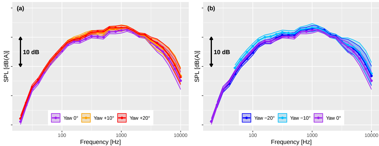
Figure 20. Turbine sound power level spectra at v = 11 m/s for positive (a) and negative (b) yaw angles. The shaded ribbon represents one standard uncertainty.
