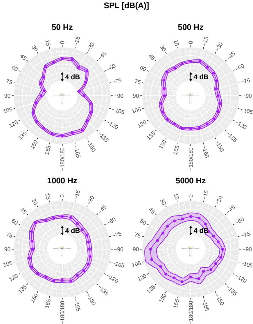
Figure 15. Directivity of A-weighted sound pressure level (SPL) at 11.5 m/s for 4 different 1/3-octave bands, without yaw misalignment. The shaded ribbon represents one standard uncertainty.
