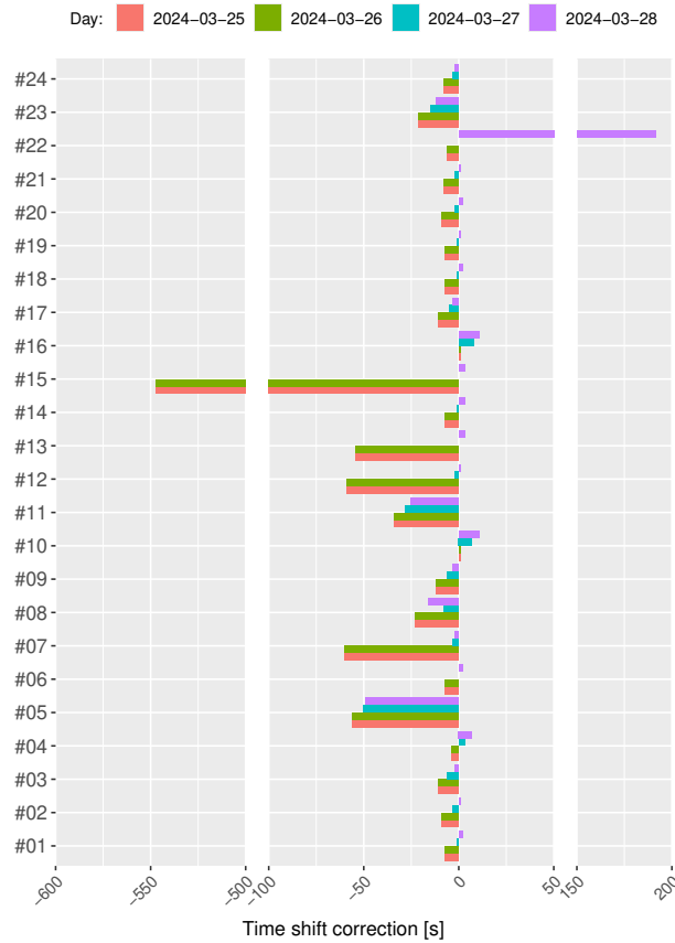
Figure 9. Time shift corrections applied for each SLM and each day of measurement. 0 seconds represents a perfect synchronization with the SCADA, a positive (resp. negative) value is found when the SLM data is ahead (resp. delayed) with respect to the SCADA.
