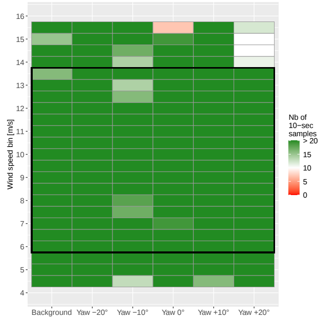
Figure 5. Raw capture matrix for the TWAIN acoustic campaign. The number of 10-second samples is shown for each wind speed bin and each yaw misalignment case. The black rectangle represents the wind speed range of interest between 6 and 13.5 m/s.
