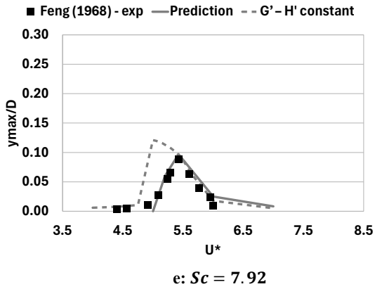
Figure 6: Oscillation amplitudes vs. U^* . Calibration of the model constants with measurements from (Feng, 1968). Predictions correspond to varying and constant G' and H' . Scruton numbers range from 2.52 to 7.92. Mass ratio m^* = 248 and Re = 1 \times 10^4 \div 5 \times 10^4 .
