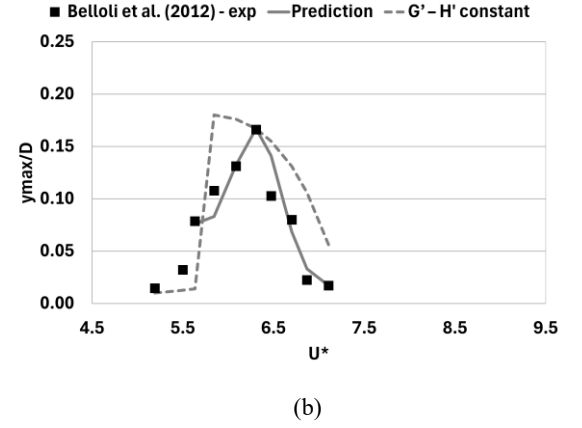
Figure 4: Oscillation amplitudes vs. U^* . Calibration of the model constants with measurements from (Belloli et al., 2012). Predictions correspond to varying and constant G' and H' . Two Sc values addressed (a) Sc = 1 , (b) Sc = 6.67 . Mass ratio m^* = 170 and Re = 4.6 \times 10^4 .
