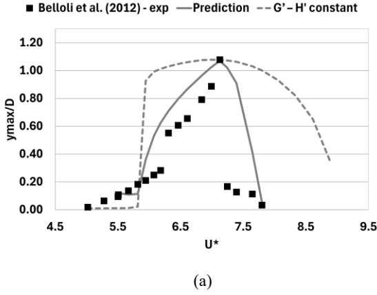
Figure 4: Oscillation amplitudes vs. U^* . Calibration of the model constants with measurements from (Belloli et al., 2012). Predictions correspond to varying and constant G' and H' . Two Sc values addressed (a) Sc = 1 , (b) Sc = 6.67 . Mass ratio m^* = 170 and Re = 4.6 \times 10^4 .
