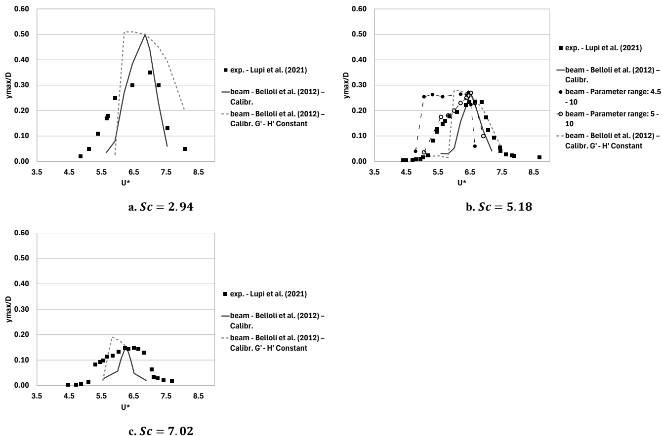
Figure 9: Maximum oscillation amplitudes normalized with respect to the reference diameter vs. U^* for the cantilever tower. Experimental results of (Lupi et al. , 2021) (solid squares) compared to predictions of the calibrated Hartlen-Currie model (continuous lines).
