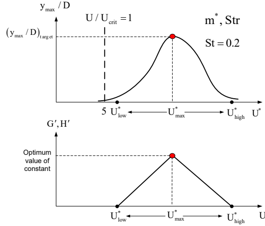
Figure 2: Schematic representation of the calibration process for the constants G', H' . Calibration is carried out for experimental y_{max}/D at U_{max}^* .
