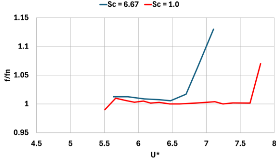
Figure 5: Frequency ratio across VIV zone for two Sc values. The plateau indicates resonance at the natural frequency, although the St shedding frequency varies. Frequencies are obtained by applying an FFT filter to the displacement of the body and obtaining the dominant frequency.
