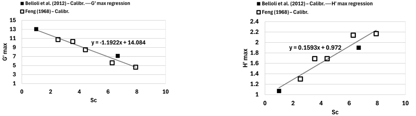
Figure 7: G'_{max} and H'_{max} across the range of Scruton numbers tested. Calibration with both experimental datasets yields very similar results and a common linear trendline is fitted.
