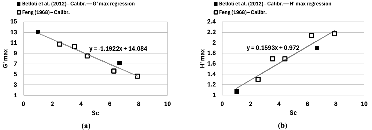
340 Figure 7: G'_{max} (a) and H'_{max} (b) across the range of Scruton numbers tested. Calibration with both experimental datasets yields very similar results and a common linear trendline is fitted.
