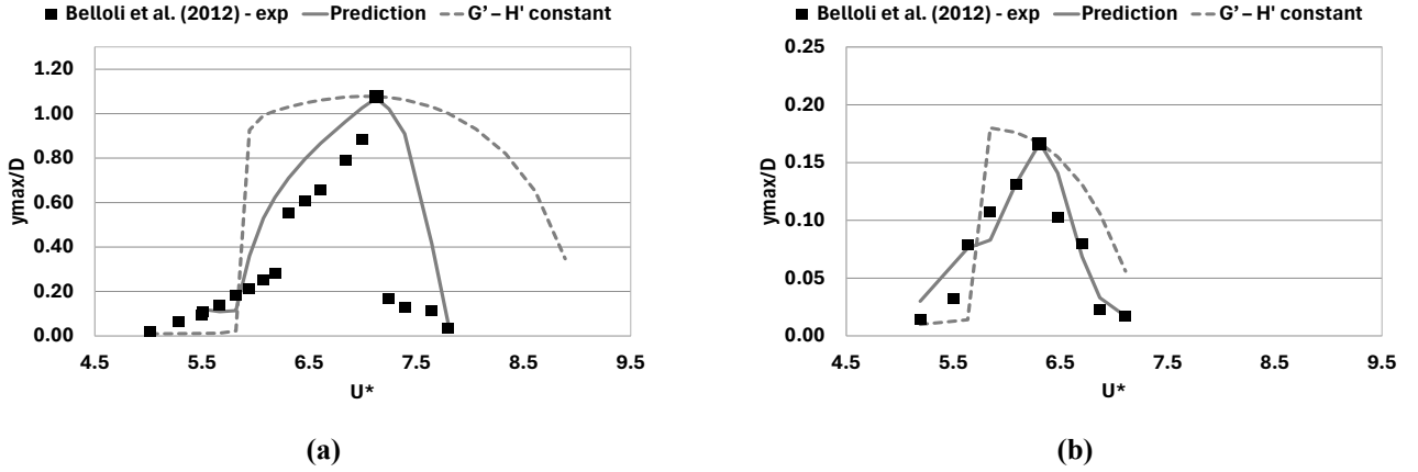
Figure 4: Oscillation amplitudes vs. U^* . Calibration of the model constants with measurements from Belloli et al. (2012). Predictions correspond to varying and constant G' and H' . Two Sc values addressed (a) Sc = 1 , (b) Sc = 6.67 . Mass ratio m^* = 170 and Re = 4.6 \times 10^4 .
