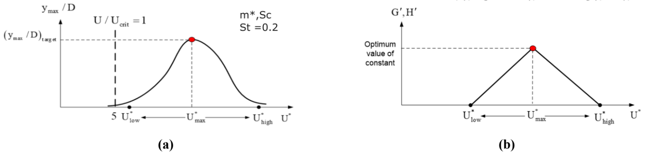
Figure 2: Schematic representation of the calibration process for the constants G', H' . Calibration is carried out for experimental y_{max}/D at U_{max}^* (a). Within the critical range the parameters are assumed to decrease linearly from their calibrated values (b).
