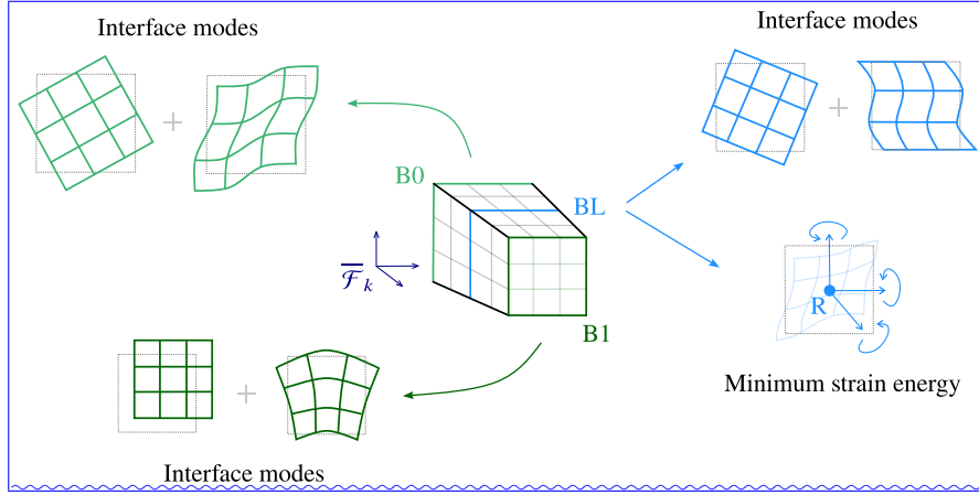
Figure 3. Interface reduction methods used for substructuring interfaces ( \text{B0B0} , \text{B1B1} ) and internal load interfaces ( \text{BLBL} ).
