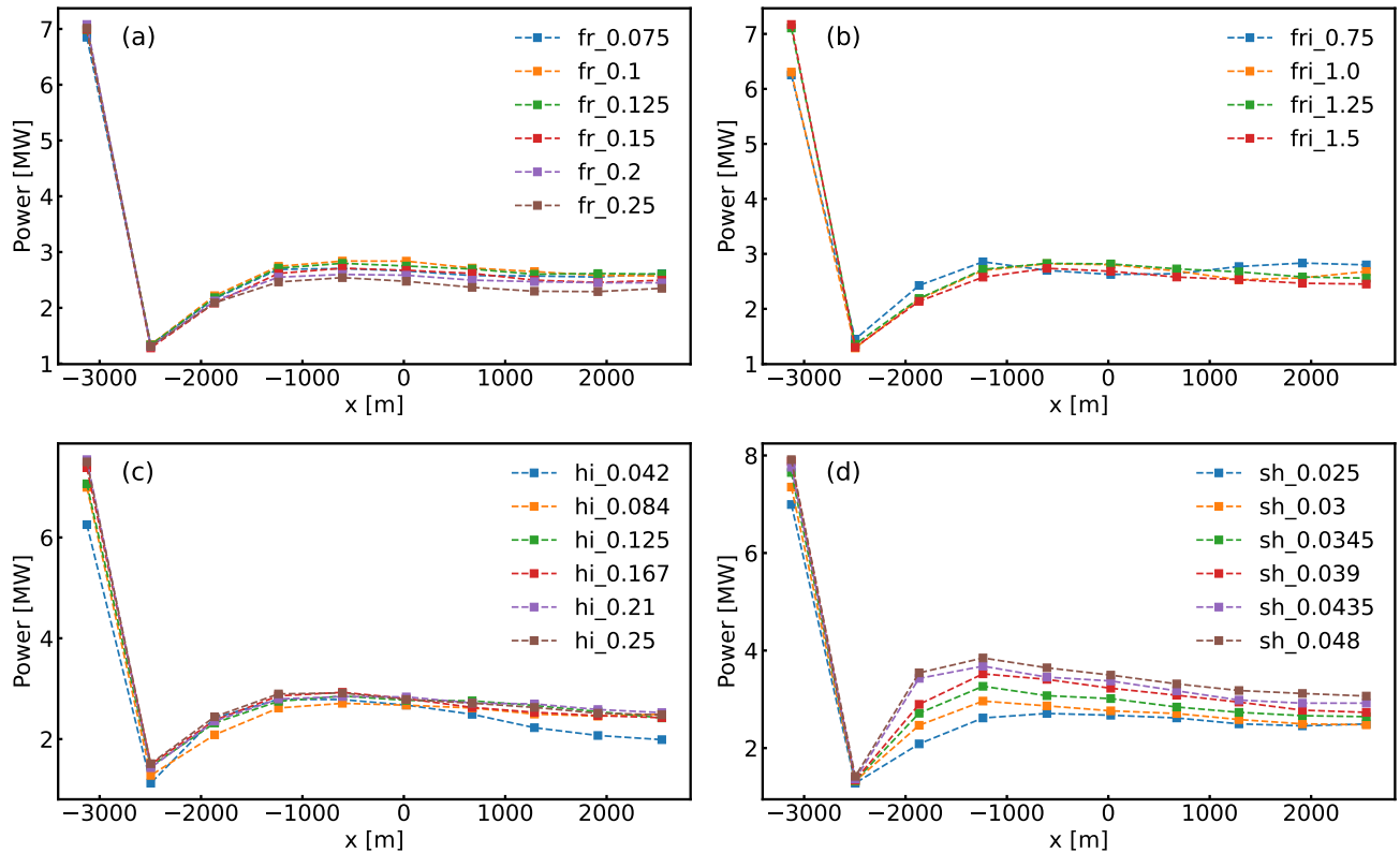
Figure 16. Temporal and row-averaged wind turbine power output as a function of Fr , Fr_i , \tilde{H}_i , and S_h .
