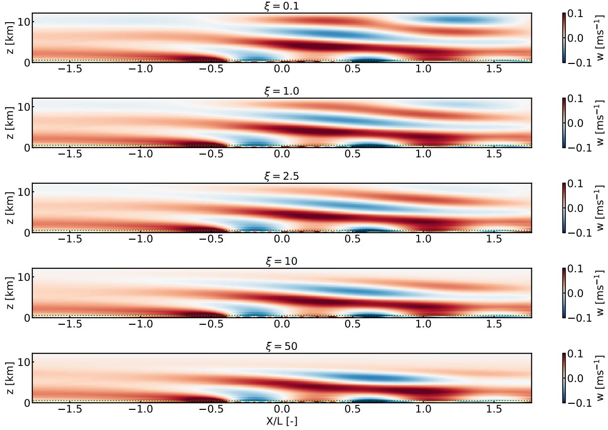
Figure 7. Contours of temporally averaged vertical velocity in a streamwise-oriented vertical plane for varying Rayleigh damping strength ( \xi ) of the T-RDL. The flow conditions are defined by Fr = 0.15 , Fr_i = 1.3 , \tilde{H}_i = 0.087 , and S_h = 0.0255 .
