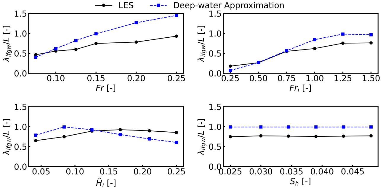
Figure 11. Interfacial wavelengths normalized with wind farm length as a function of Fr , Fr_i , \tilde{H}_i , and S_h . A comparison of wavelengths measured from LES data with those calculated with the deep-water approximation, where the ABL depth is considered large enough and therefore insignificant.
