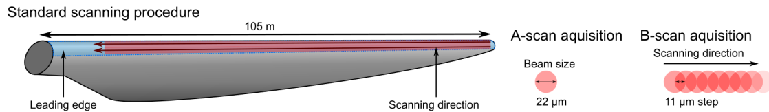
Figure 13. Schematic of the proposed standard procedure for blade inspection.
