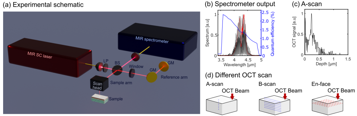
Figure 4. (a) 3D representation of the MIR OCT system, SC: supercontinuum, LP: 3.2 \mu\text{m} long pass filter, BS: beam splitter, GM: gold mirror. (b) Reference spectrum in red, measured interference spectrum in black, upconversion efficiency in blue, and (c) the corresponding calculated A-scan. (d) Schematic of the different OCT scans used in this article.
