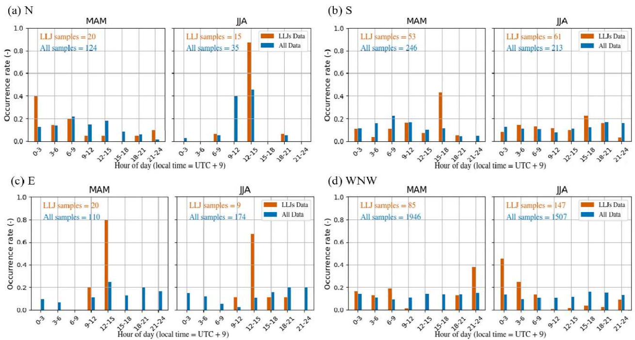
Figure 75: Hour-of-day distribution of LLJ occurrences.
