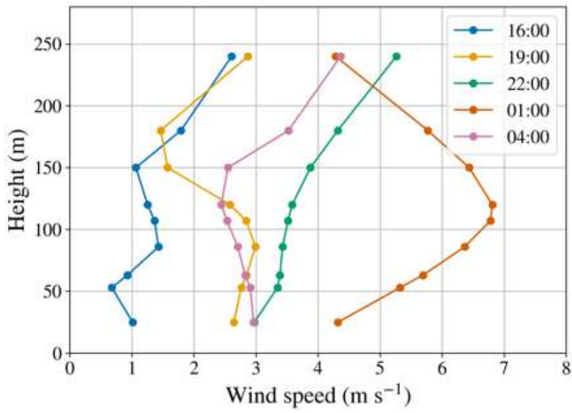
480 Figure 12: Vertical profiles of wind speed at selected times on 11 July 2024.
