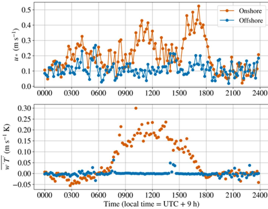
530 Figure 149: Time series of friction velocity and covariance of vertical velocity and temperature at the onshore and offshore sites on 2 May 2024
