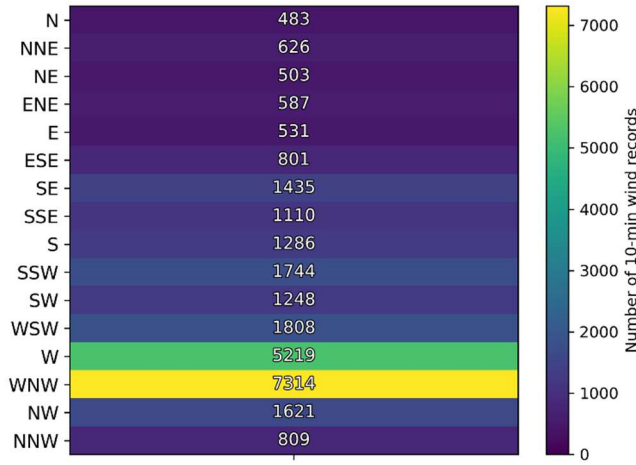
Figure 6: Frequencies of LLJs occurrences by wind direction. The color scales differ between panels. In panel (a), the values represent the number of 10-min wind records for each wind direction. In panel (b), values in parentheses indicate the LLJ occurrence rate (%), defined as the ratio of LLJ records to the total number of wind records for each direction. Wind direction labels follow the meteorological convention (e.g., N = north, WNW = west-northwest). Table 3: Occurrence frequencies of LLJs by wind direction and season.
