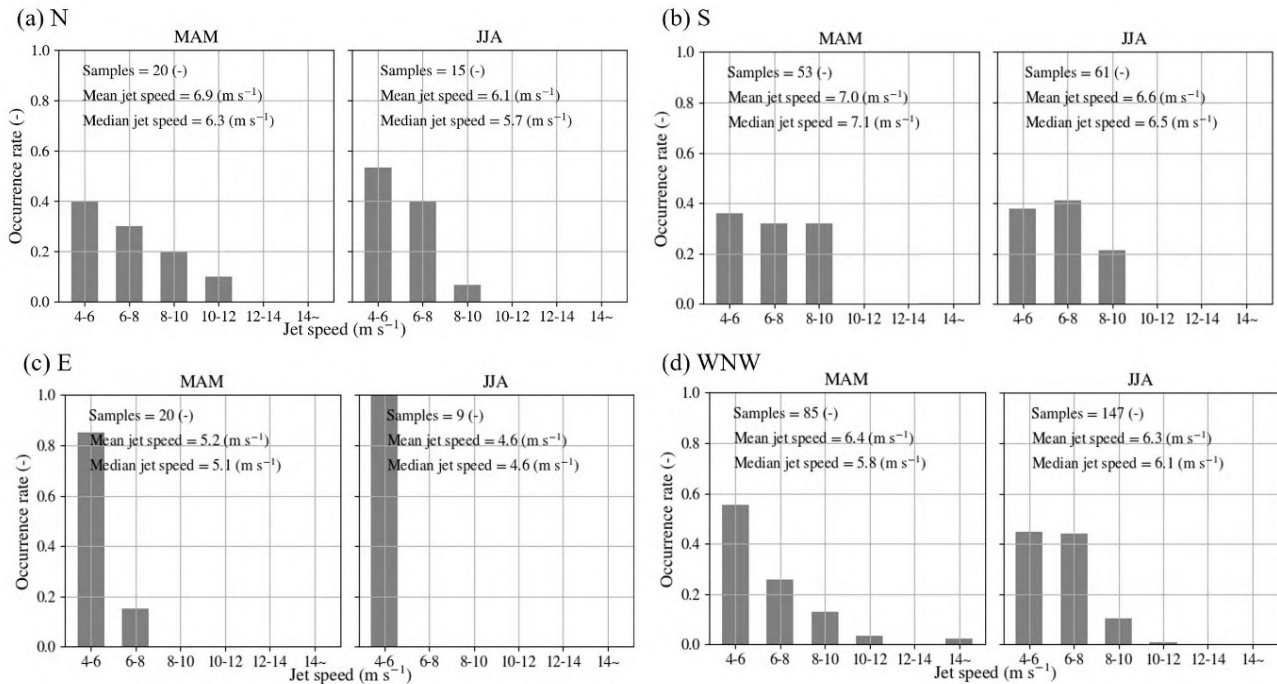
Figure 86: LLJ core wind speeds by wind direction in spring and summer.
