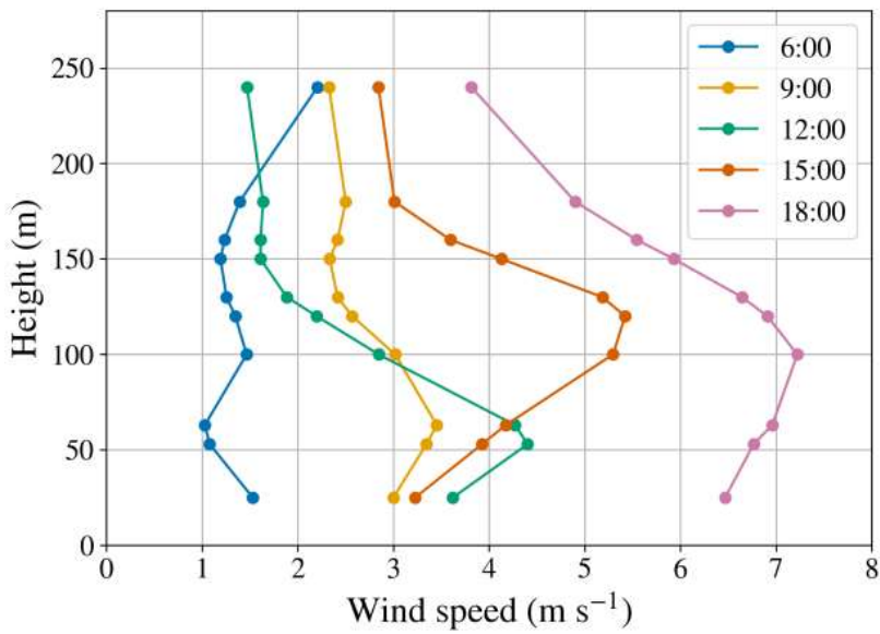
350 Figure 10: Vertical profiles of wind speed at selected times on 2 May 2024.
