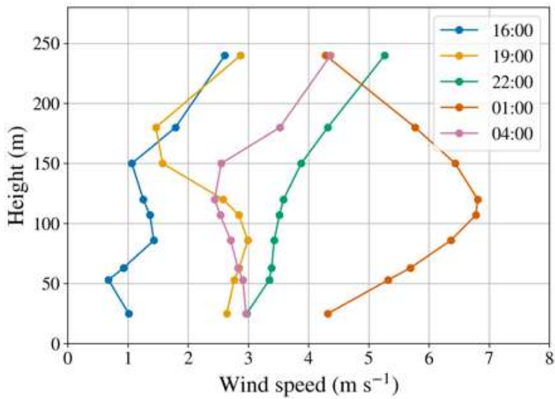
355 Figure 12: Vertical profiles of wind speed at selected times on 11 July 2024.
