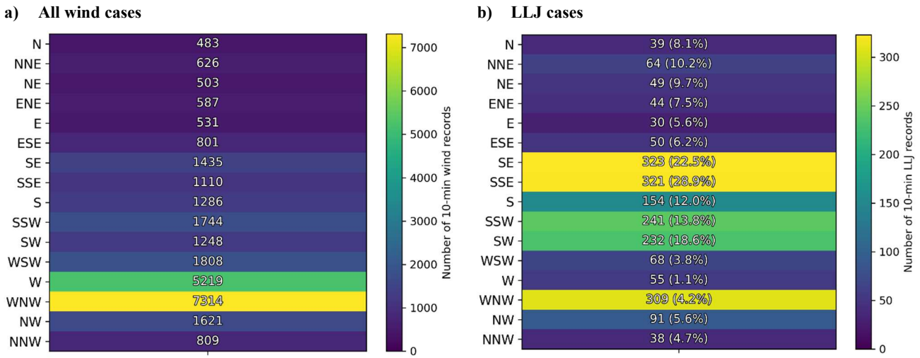
Figure 6: Frequencies of LLJs occurrences by wind direction. The color scales differ between panels. In panel (a), the values represent the number of 10-min wind records for each wind direction. In panel (b), values in parentheses indicate the LLJ occurrence rate (%), defined as the ratio of LLJ records to the total number of wind records for each direction. Wind direction labels follow the meteorological convention (e.g., N = north, WNW = west-northwest).
