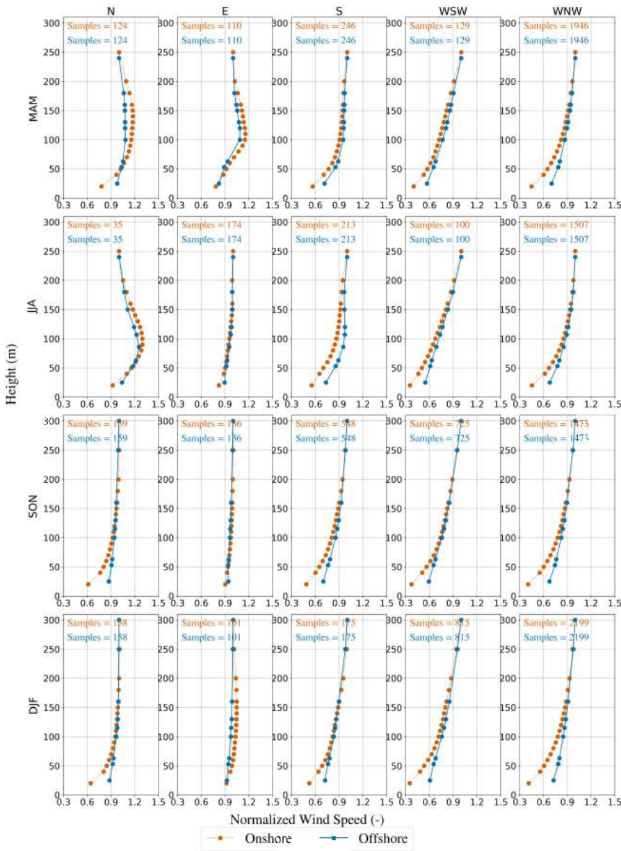
220 Figure 5: Vertical profiles of normalized wind speed averaged by wind direction and season. The normalized wind speed was defined as the wind speed at each height divided by the wind speed at the highest available measurement height for each profile. The normalization was applied to each individual profile prior to averaging. The sample size indicates the number of 10-min averaged data points that fall within each wind direction sector in the one-year dataset. Wind direction labels follow meteorological convention (e.g., N = north, WNW = west-northwest). Seasons are abbreviated as MAM (March-May), JJA (June-August), SON (September-November), and DJF (December-February).
