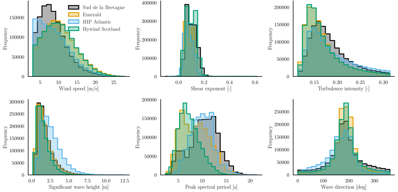
Figure 14. Comparison of the site conditions at the four floating wind sites considered in this study (Table A1).
