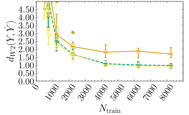
(b) d_{W2} for the predicted conditional pdf
