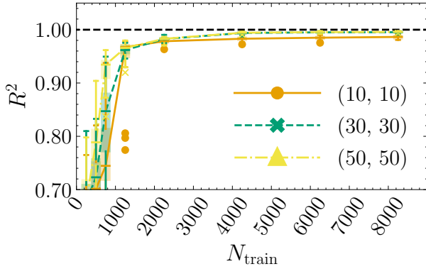
(a) R^2 values for the predicted mean
