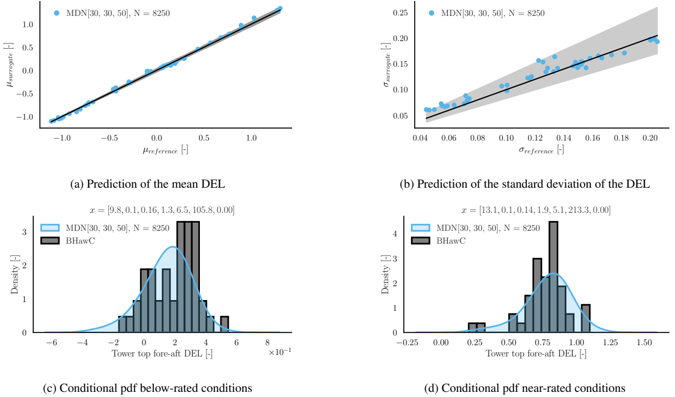
Figure 11. Load predictions using MDN for the tower top fore-aft DEL (normalized). Figure (a) shows the surrogate predicted conditional mean at the test locations vs. the conditional mean calculated using BHawC. Figure (b) shows the predicted and reference standard deviations of the conditional pdf. Figures (c) and (d) compare the conditional pdf plots between the surrogate and the simulation at below-rated and near-rated conditions, respectively. The values in vector x denote: [U_{\text{ref}}, \alpha, TI, H_s, T_p, W_{\text{dir}}, Y_{\text{aw}}] with units specified in Table 4.
