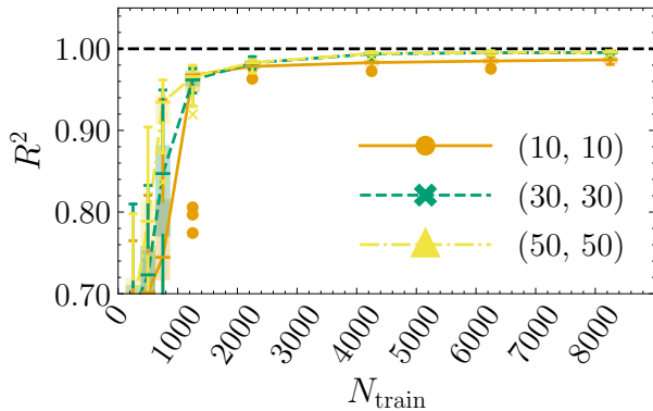
(a) R^2 values for the predicted mean
