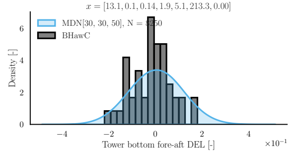
(d) Conditional pdf near-rated conditions
