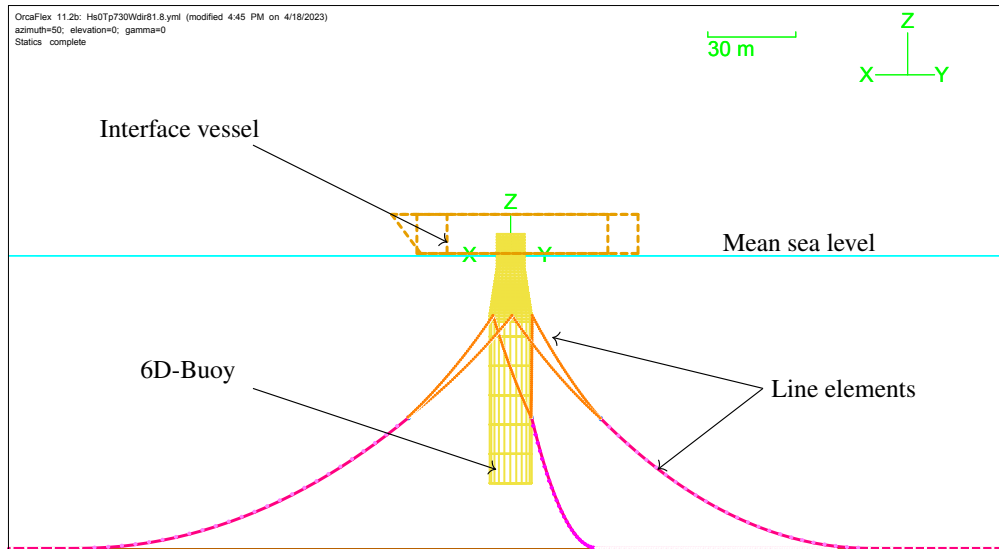
Figure 3. Schematic of the OrcaFlex simulation elements.
