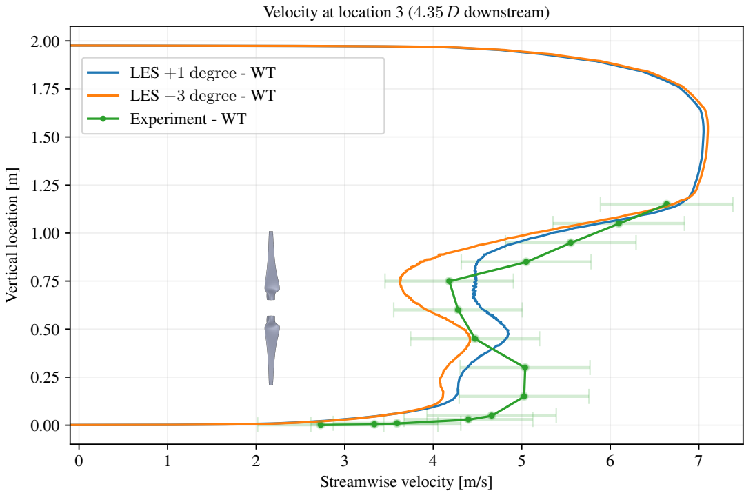
Figure 21. Velocity profile comparing the LES simulation using two pitch angles with the experiment at location 3 ( 4.35 D 4.35 D downstream of the wind turbine).
