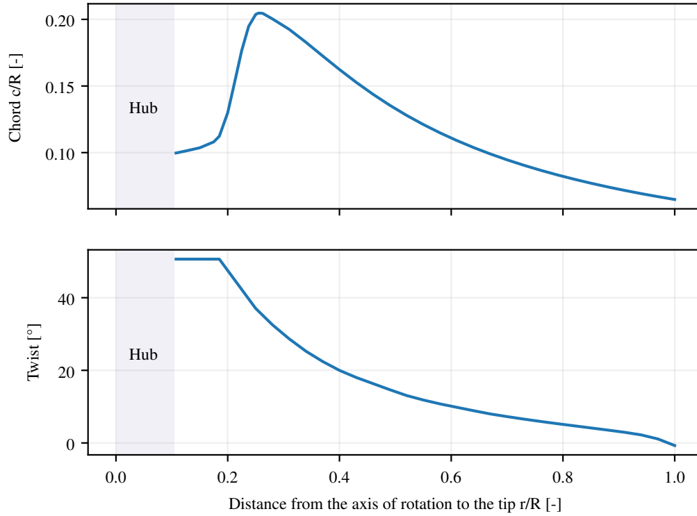
Figure 5. Blade design parameter parameters for the TWIST wind turbine.
