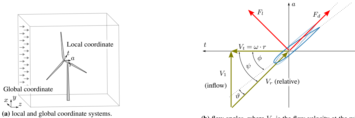
Figure 16. Coordinate systems (a), and local wind speed and directions around the blade (b).
