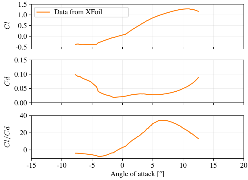
Figure 17. coefficients Coefficients of lift and drag obtained from XFOil for the airfoil SD7037-092-88.
