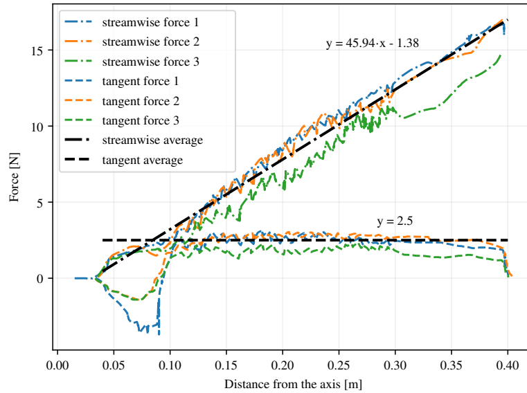
Figure 22. 3D-CAD Distribution of forces along the deformed blade ,with indications for in the forces applied to its stationary frame of reference from the LES simulation using the cALM.
