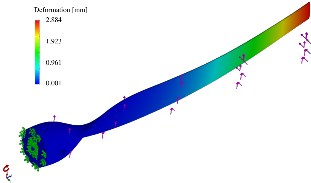
Figure 23. 3D CAD of the deformed blade, with indications for the forces applied to it.
