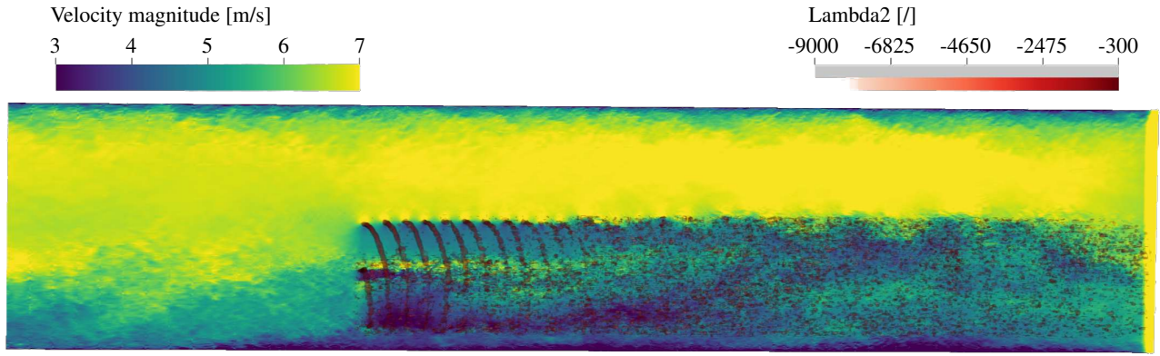
Figure 18. Field of instantaneous velocity magnitude using cALM in the vertical symmetry plane passing through the hub of the wind turbine, on which a lambda2 criterion isocontour is overlaid, highlighting the vortices from the wake.
