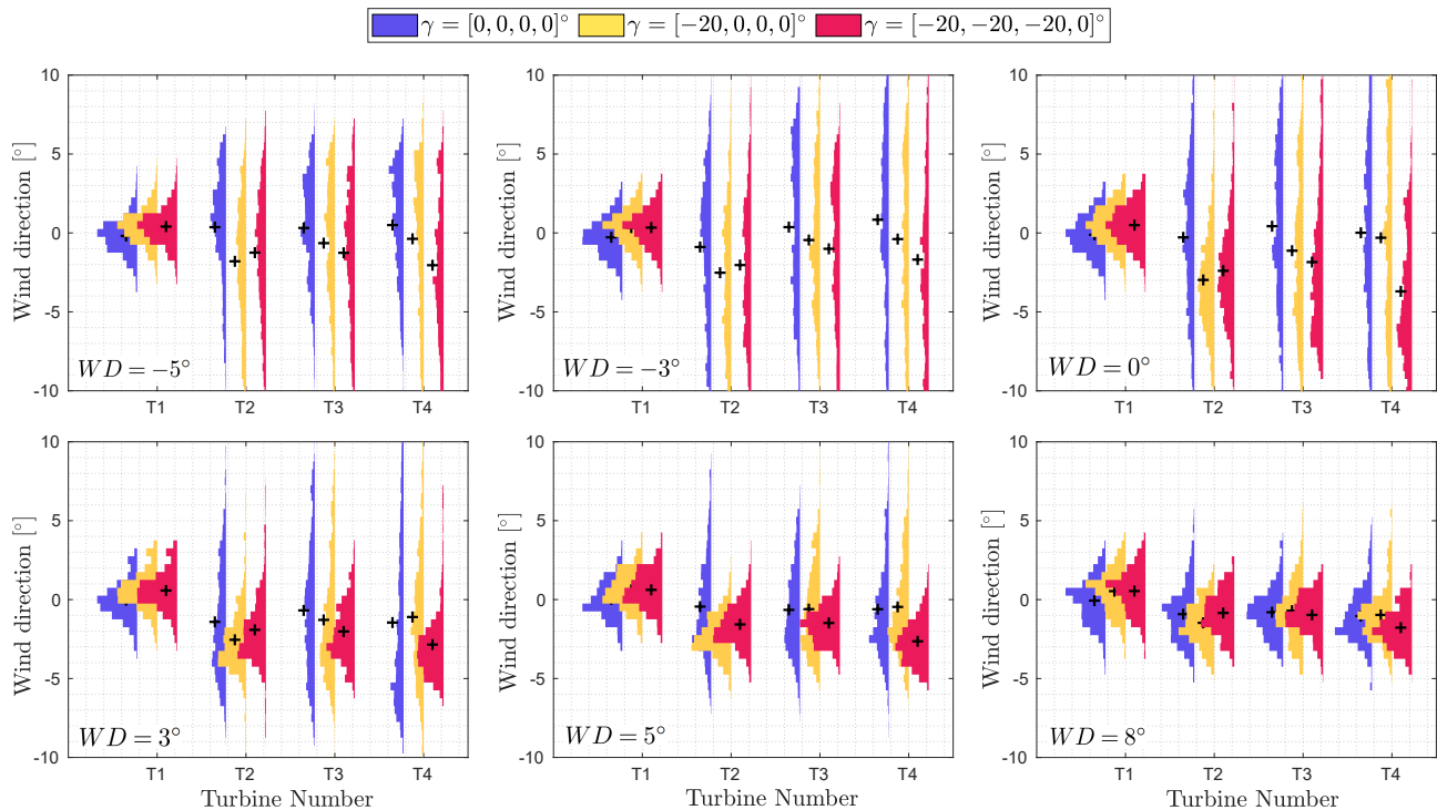
Figure 5. Area-normalised histograms of wind direction measured \pm R-0.5D upstream of each turbine location for all yaw scenarios and for each inflow wind direction. Black crosses indicate the mean of each distribution.
