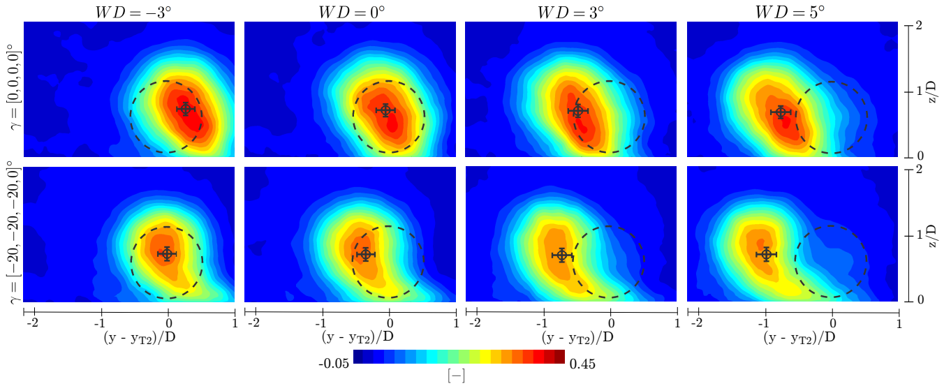
Figure 3. Contour plots using cross-stream plane at 1R in front of Turbine 2, showing mean normalised velocity deficit, \frac{U(z)_{in} - U}{U(z)_{in}} velocity. Mean wake centre position and error bars showing standard deviation of wake centre in black. Dashed circle represents the rotor position and area of Turbine 2. Top row: baseline cases without yaw; bottom row: first three turbines yawed. From left to right: wind directions of -3^\circ , 0^\circ , 3^\circ , 5^\circ . Planes oriented as seen from behind.
