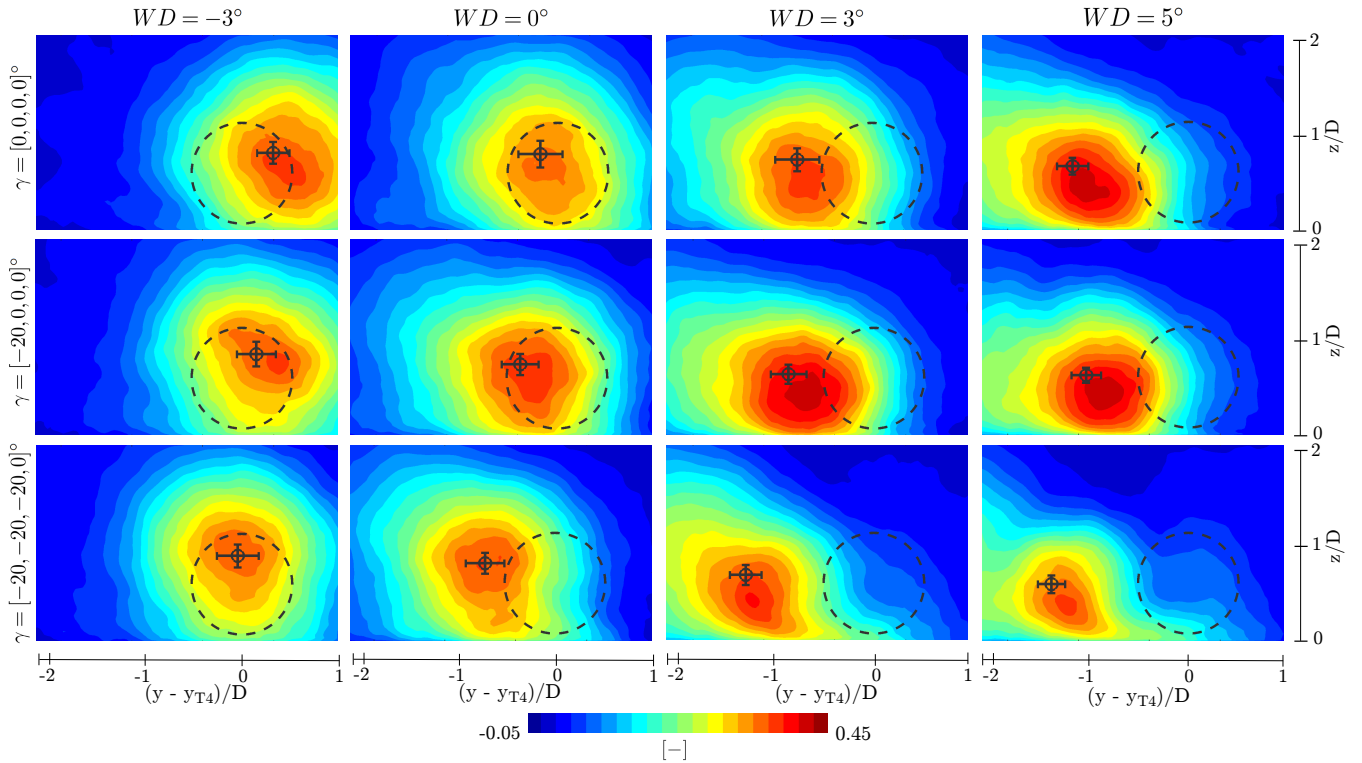
Figure 4. Contour plots using cross-stream plane at \pm R in front -0.5D in front of Turbine 4, showing mean normalised velocity deficit, \frac{U(z)_{in} - U}{U(z)_{in}} ( \frac{U(z)_{in} - U}{U(z)_{in}} velocity). Mean wake centre position and error bars showing standard deviation of wake centre in black. Dashed circle represents the rotor position and area of Turbine 4. Top row: baseline cases without yaw; middle row: first turbine yawed; bottom row: first three turbines yawed. From left to right: wind directions of -3^\circ , 0^\circ , 3^\circ , 5^\circ . Planes oriented as seen from behind.
