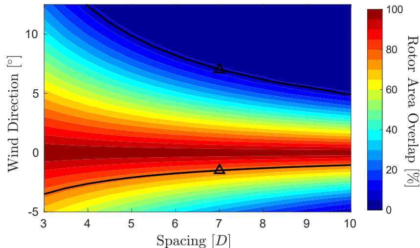
Figure 11. Percentage overlap of two aligned row turbine rotor areas at different spacings and for different wind directions. Marker-Markers shows the zero crossing of \Delta\overline{P_{farm}} as predicted in Figure 10B, for the spacing 7D simulated here. Lines show a constant rotor overlap percentage calculated for each marker point.
