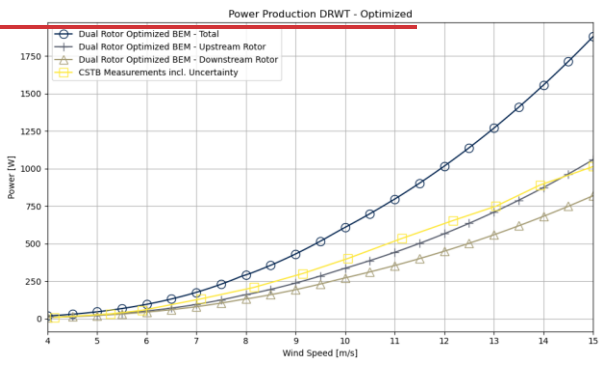
Figure 108: Power production of optimized CR-DRWT.
