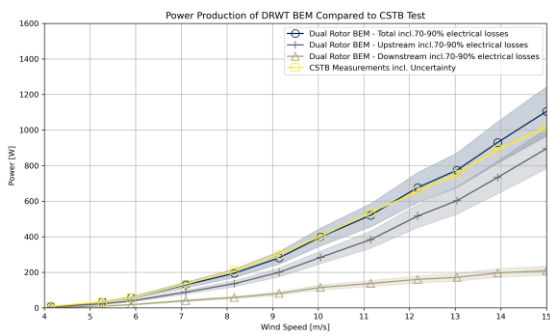
365 Figure 65: Results of power production during the wind tunnel test compared to BEM results. The figure shows both rotors individually, the CR-DRWT and the wind tunnel test data.
