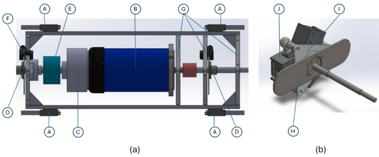
Figure 1: Overview of the mechanical lay-out of the CR-DRWT. (a) Nacelle Overview, (b) Pitch Mechanism. (In which A: Linear Actuators, B: Generator, C: Generator Cap, D: Disc Brakes, E: Slip Ring, F: Plate with external bearing, G: Plates with internal bearing, H: Push/Pull Plate, I: Traingular Place, J: Blade Holders.) Taken from (Adema et al., 2025).
