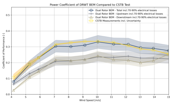
Figure 76: Results of the coefficient of performance during the wind tunnel test compared to BEM results. The figure shows both rotors individually, the CR-DRWT and the wind tunnel test data.
