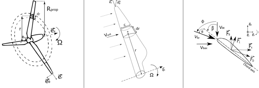
Figure 43: BEM parameters definition. Left: global wind turbine, middle: Blade element definition, right: flow velocities and forces seen by a blade element. Adapted from figures 2 to 4 from (Amoretti et al., 2023).
