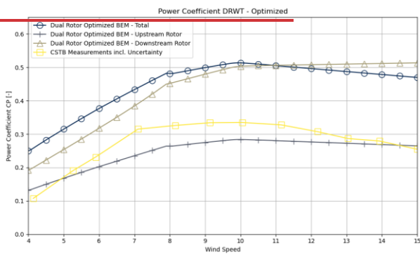
405 Figure 119: Power coefficient of optimized CR-DRWT.
