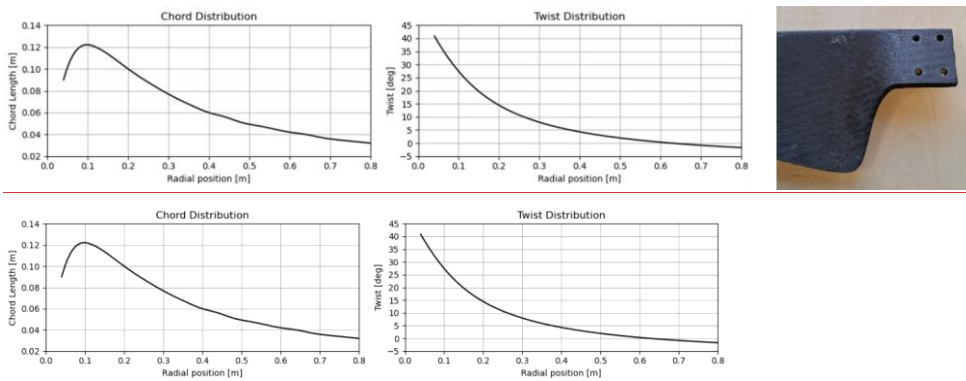
Figure 21: Aerodynamic design of both rotors of the DRWT. Left: the chord distribution. Right Middle: the twist distribution. Right: Zoom in on the root section of the blades.
