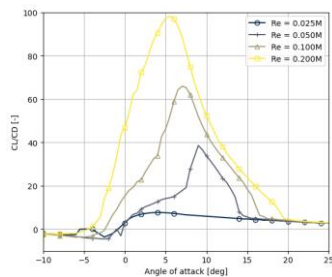
Figure 54: Profile aerodynamics of SG6043 airfoil at N_{crit} = 9 .
