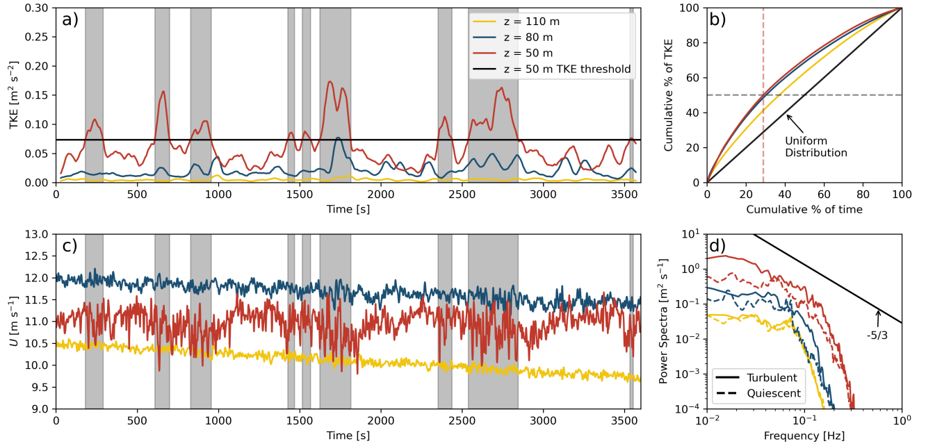
Figure 6. (a) Time-series and (b) CDF-cumulative distribution function of TKE at various heights within the rotor disk for the strongly stable regime 5D upwind of the wind farm on the inner domain. (c) Time-series and (d) power spectra of wind speed at the same heights as in (a) and (b). The dashed lines in (b) pinpoint the the-cumulative percentage of time it takes until 50% of the TKE occurs at a height of 50 m . The periods highlighted in gray are “turbulent” while other periods are “quiescent”. In (d), the -5/3 inertial subrange power law is provided in black for reference.
