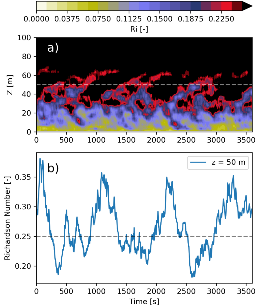
Figure B1. (a) Time-height contour of the gradient Richardson number ( Ri ) at 5D upwind of the wind farm on the inner domain during the analysis period emphasizing the critical Richardson number value of 0.25. (b) Time-series of Ri at z = 50 m with a dashed line at Ri = 0.25 corresponding to the critical Richardson number.
