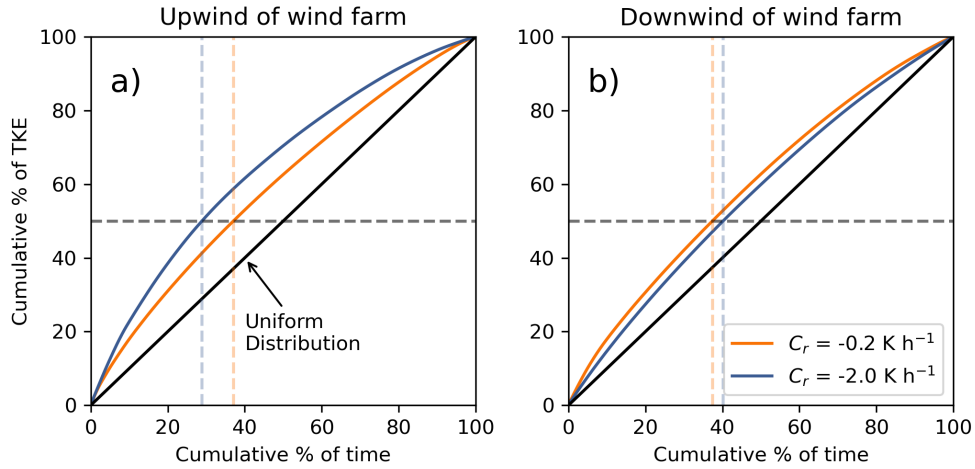
Figure 11. Cumulative distribution function of TKE (a) 5D upwind ( x = -5D ) and (b) 10D downwind ( x = 26D ) of the wind farm for each stability regime at z = 50 \text{ m} . The dashed lines pinpoint the cumulative percentage of time it takes until 50% of the TKE occurs.
