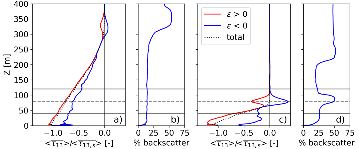
Figure 5. Planar- and time-averaged vertical profiles of normalized total momentum flux (resolved + modeled) for the (a) weakly stable and (c) strongly stable regime for the DRM closure at 8 m resolution conditionally averaged based on the sign of the SFS dissipation rate (negative indicating backscatter). Percentage of backscatter in the SFS dissipation rate for a given height for the (b) weakly and (d) strongly stable regimes. Note that results shown are for the outer domain without wind turbines. The solid horizontal lines represent the bottom and top of the rotor layer while the dashed line represents hub-height.
