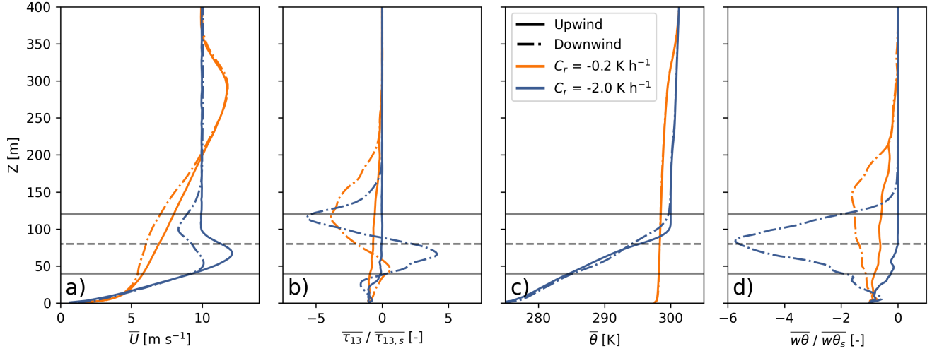
Figure 12. Vertical profiles of (a) wind speed, (b) streamwise vertical momentum flux, (c) potential temperature, and (d) vertical heat flux, 5D upwind ( x = -5D ) and 5D downwind ( x = 21D ) of the farm for each stability regime. The solid horizontal lines represent the bottom and top of the rotor layer while the dashed line represents hub-height.
