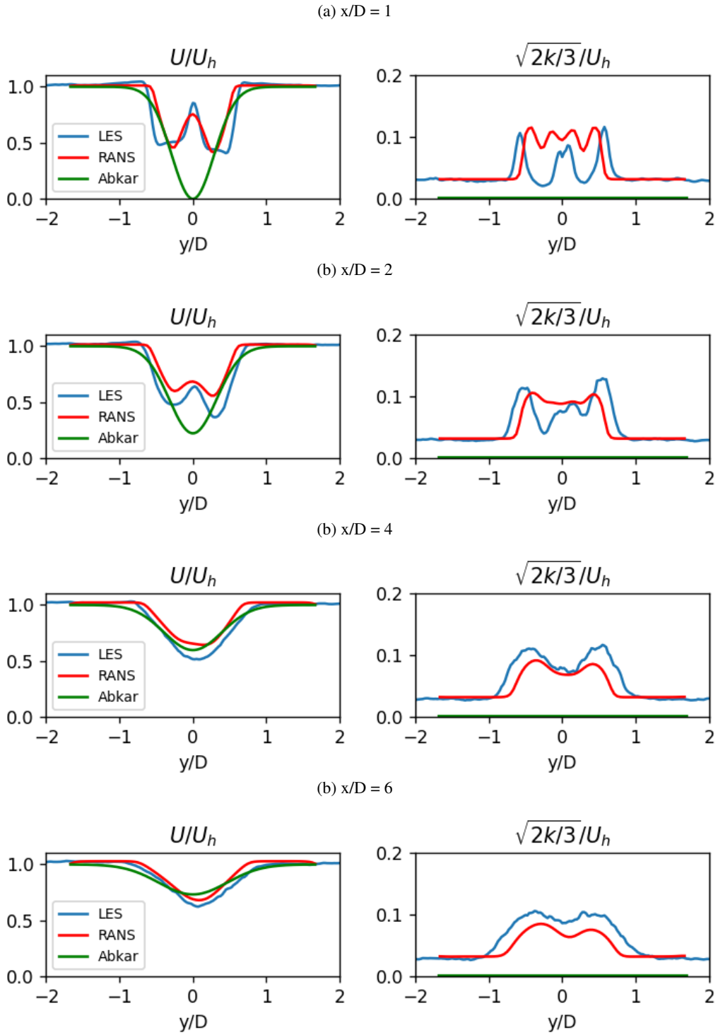
Figure 19. Hub-height profiles of the normalized velocity and normalized TKE \sqrt{2k/3}/U_h for the single turbine wake in the Low WS ABL conditions, as computed by the LES, SANDWake3D RANS, and Abkar et al model.
