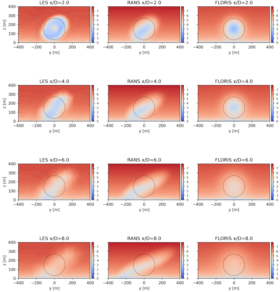
Figure 4. Comparison of the streamwise velocity u(y, z) for the Low WS inflow condition, as computed by Kynema-SGF LES, SAND-Wake3D RANS, and FLORIS empirical Gaussian methods. Contours of u(y, z) are plotted with units of meters/second at distances x/D = 2, 4, 6, 8 downstream of the turbine. The dashed circle corresponds to the location of the rotor disk of the IEA 15MW reference turbine.
