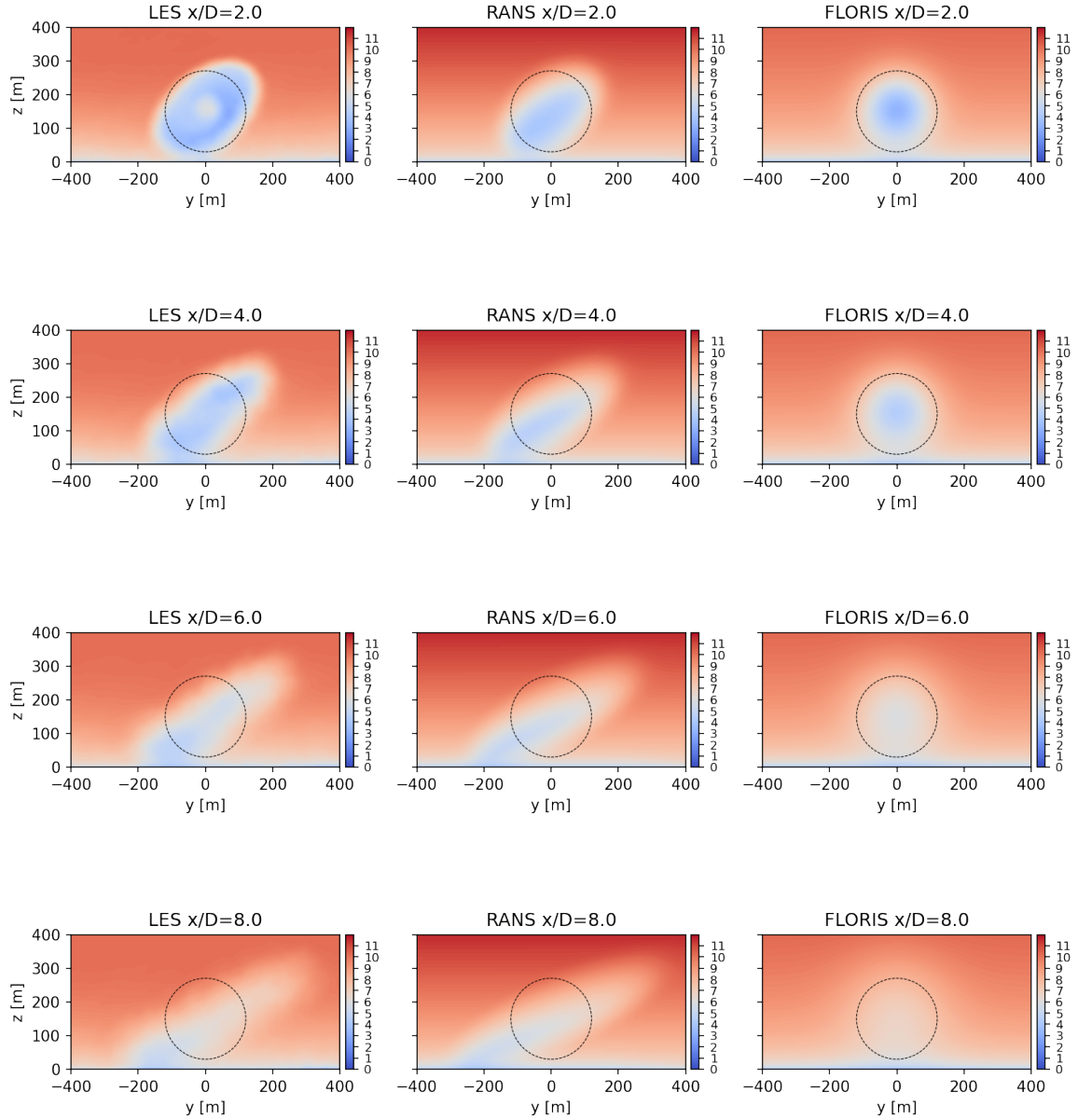
Figure 5. Comparison of the streamwise velocity u(y, z) for the Med WS inflow condition, as computed by Kynema-SGF LES, SAND-Wake3D RANS, and FLORIS empirical Gaussian methods. Contours of u(y, z) are plotted with units of meters/second at distances x/D = 2, 4, 6, 8 downstream of the turbine. The dashed circle corresponds to the location of the rotor disk of the IEA 15MW reference turbine.
