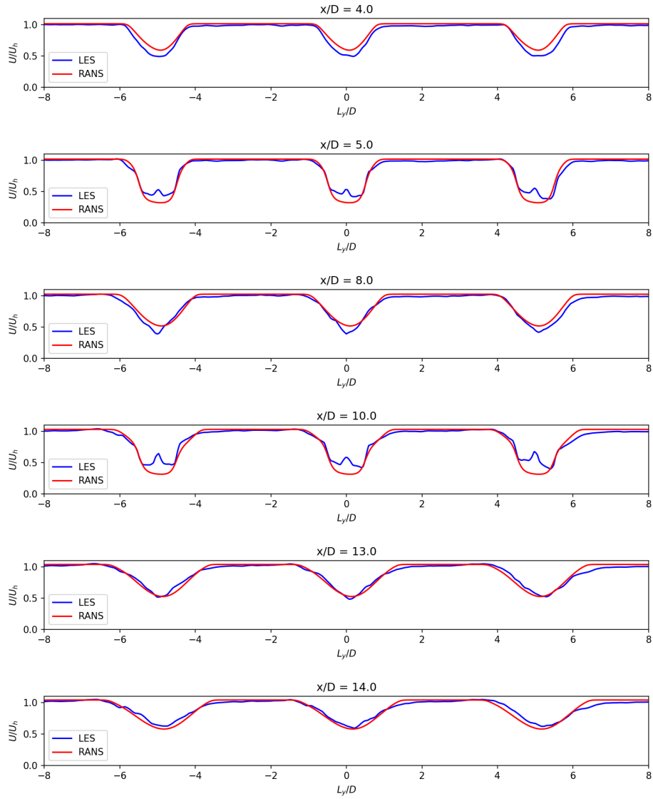
Figure 17. Hub-height profiles of the normalized velocity the 9-turbine wind farm configuration in the Med WS ABL conditions, as computed by the Kynema-SGF LES and SANDWake3D RANS codes. Note that all streamwise distances are measured from the first turbine row at x/D = 0 , the second turbine row is located at x/D = 5 , and the third at x/D = 10 . Note that L_y is the lateral coordinate measured from the center turbine.
