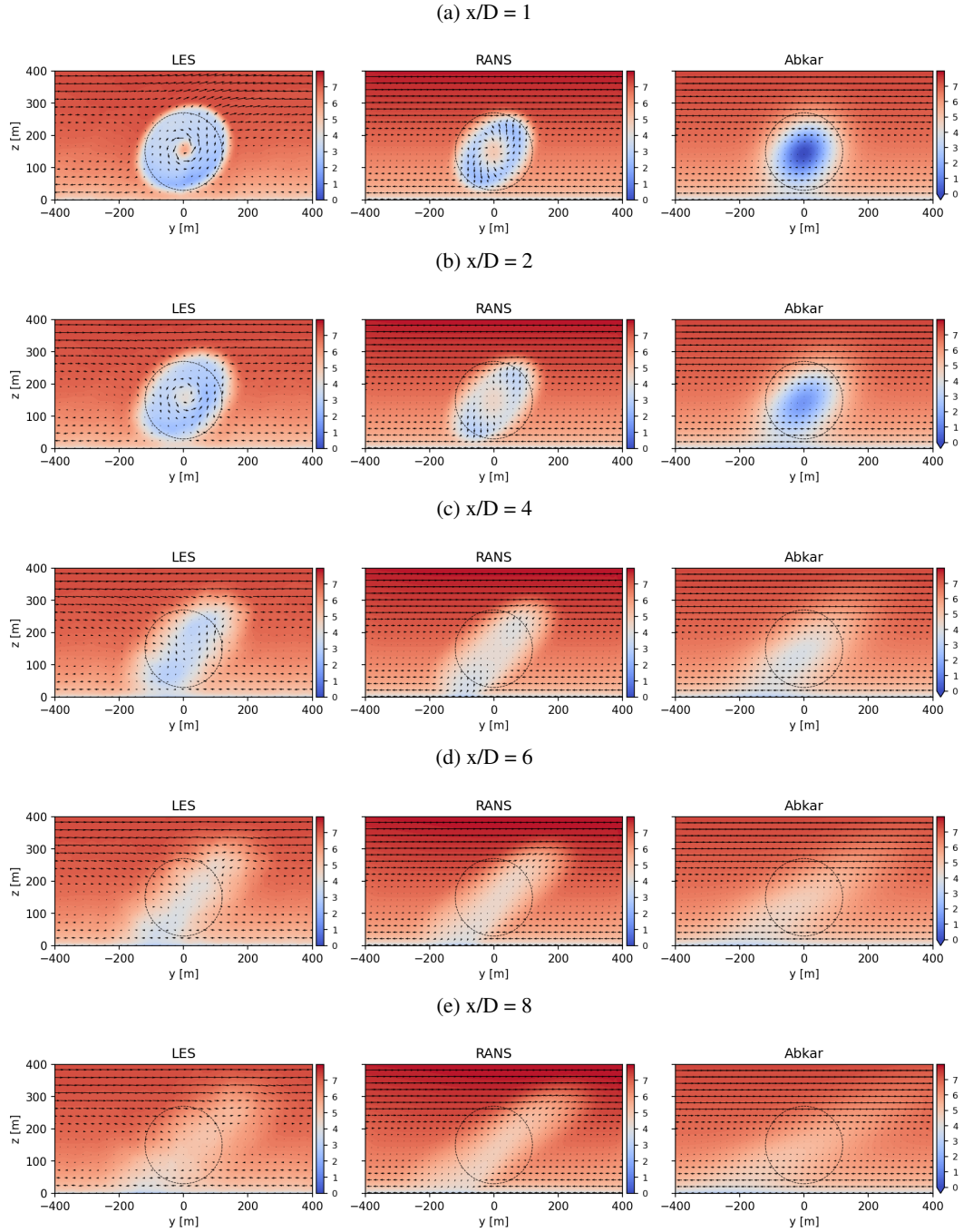
Figure 18. Comparison of the streamwise velocity for the Low WS case computed by the LES, RANS, and semi-analytic approach of Abkar et al Abkar et al. (2018). Contours of u(y, z) are plotted with units of meters/second at distances x/D = 2, 4, 6, 8 downstream of the turbine. The dashed circle corresponds to the location of the rotor disk of the IEA 15MW reference turbine.
