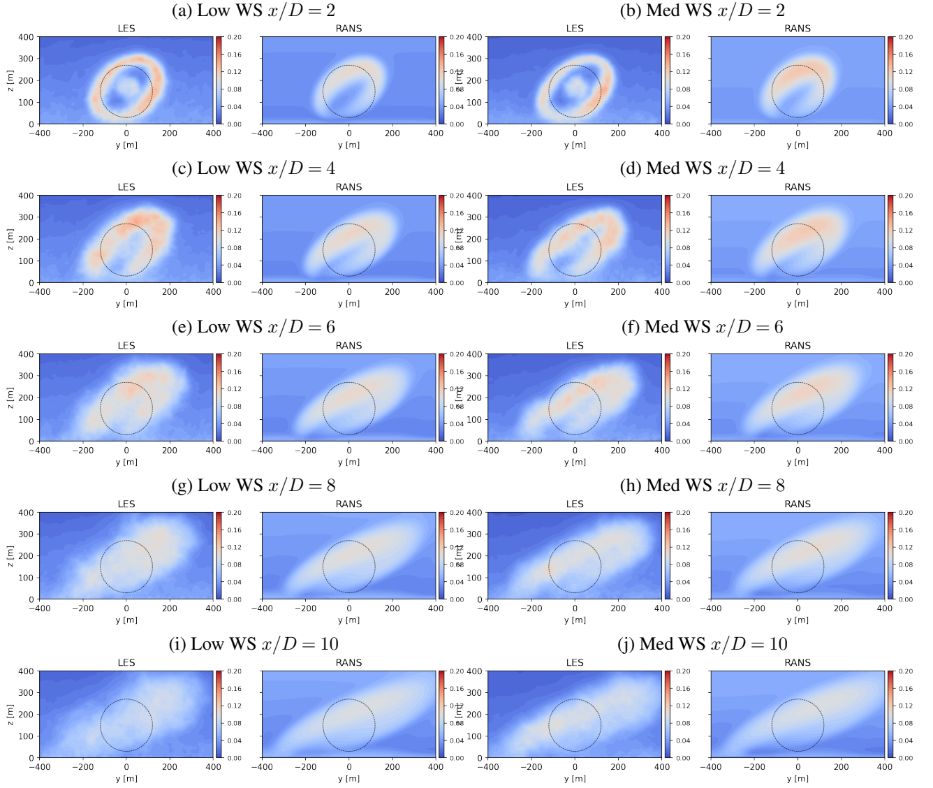
Figure 6. Comparison of the normalized turbulent kinetic energy for the Low and Med WS inflow condition, as computed by Kynema-SGF LES and SANDWake3D RANS methods. Contours of nondimensionalized TKE are plotted at distances x/D = 2, 4, 6, 8, 10 downstream of the turbine. The dashed circle corresponds to the location of the rotor disk of the IEA 15MW reference turbine.
