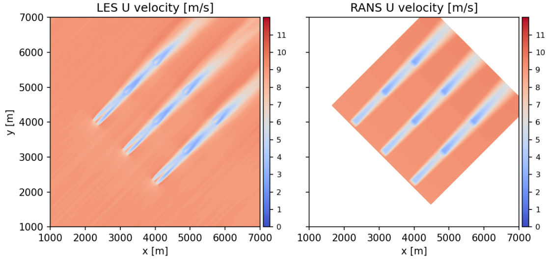
Figure 14. The streamwise velocity on the hub-height plane for the 3 row turbine wind farm configuration in the Med WS inflow, as computed by Kynema-SGF LES and SANDWake3D RANS methods. The 9 IEA 15 MW turbines are spaced 5D apart in both the lateral and streamwise directions.
