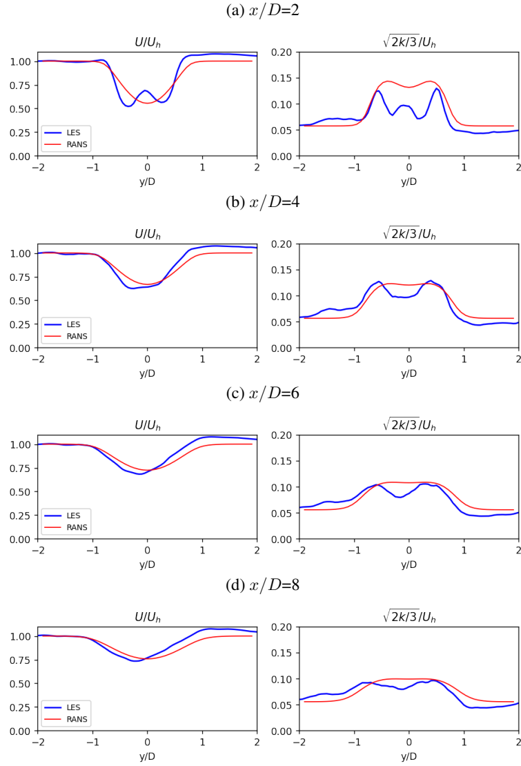
Figure 10. Comparison of the normalized hub-height velocity and turbulent kinetic energy wake profiles for the onshore convective ABL case with the NREL5MW turbine.
