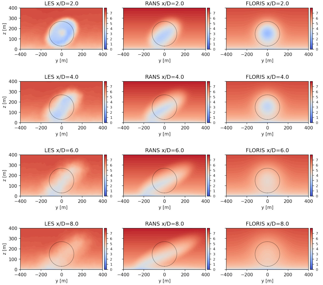
Figure 4. Comparison of the streamwise velocity u(y, z) for the Low WS inflow condition, as computed by Kynema-SGF LES, SAND-Wake3D RANS, and FLORIS empirical Gaussian methods. Contours of u(y, z) are plotted with units of meters/second at distances x/D = 2, 4, 6, 8 downstream of the turbine. The dashed circle corresponds to the location of the rotor disk of the IEA 15MW reference turbine.
