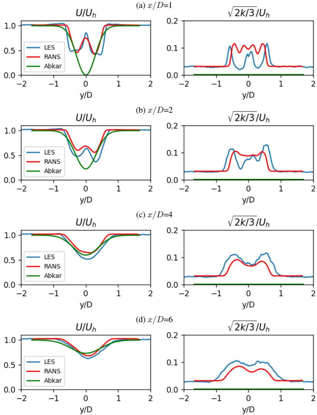
Figure 19. Hub-height profiles of the normalized velocity and normalized TKE \sqrt{2k/3}/U_h for the single turbine wake in the Low WS ABL conditions, as computed by the LES, SANDWake3D RANS, and Abkar et al model.
