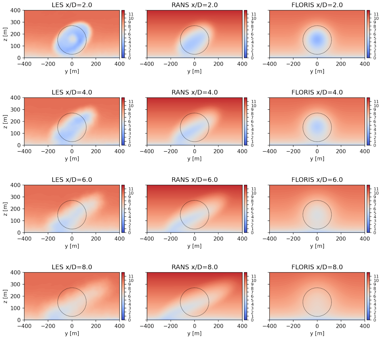
Figure 5. Comparison of the streamwise velocity u(y, z) for the Med WS inflow condition, as computed by Kynema-SGF LES, SAND-Wake3D RANS, and FLORIS empirical Gaussian methods. Contours of u(y, z) are plotted with units of meters/second at distances x/D = 2, 4, 6, 8 downstream of the turbine. The dashed circle corresponds to the location of the rotor disk of the IEA 15MW reference turbine.
