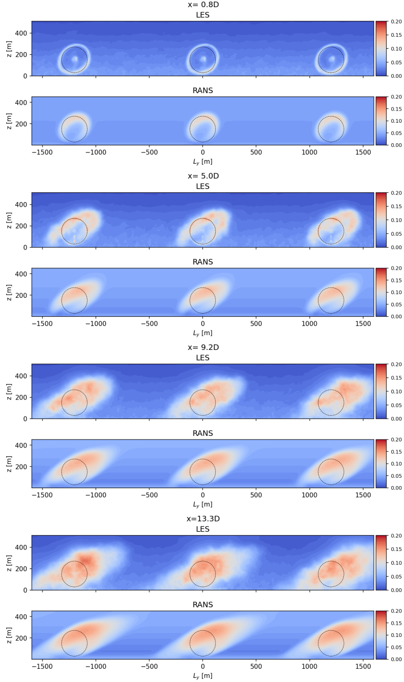
Figure 16. Rotor plane contours of the normalized TKE \sqrt{2k/3}/U_h for the 9-turbine wind farm configuration in the Med WS inflow. Note that all streamwise distances are measured from the first turbine row at x/D = 0 , the second turbine row is located at x/D = 5 , and the third at x/D = 10 . Note that L_y is the lateral coordinate measured from the center turbine.
