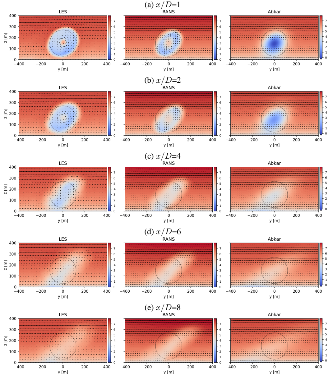
Figure 18. Comparison of the streamwise velocity for the Low WS case computed by the LES, RANS, and semi-analytic approach of Abkar et al. (2018). Contours of u(y, z) are plotted with units of meters/second at distances x/D = 1, 2, 4, 6, 8 downstream of the turbine. The dashed circle corresponds to the location of the rotor disk of the IEA 15MW reference turbine.
