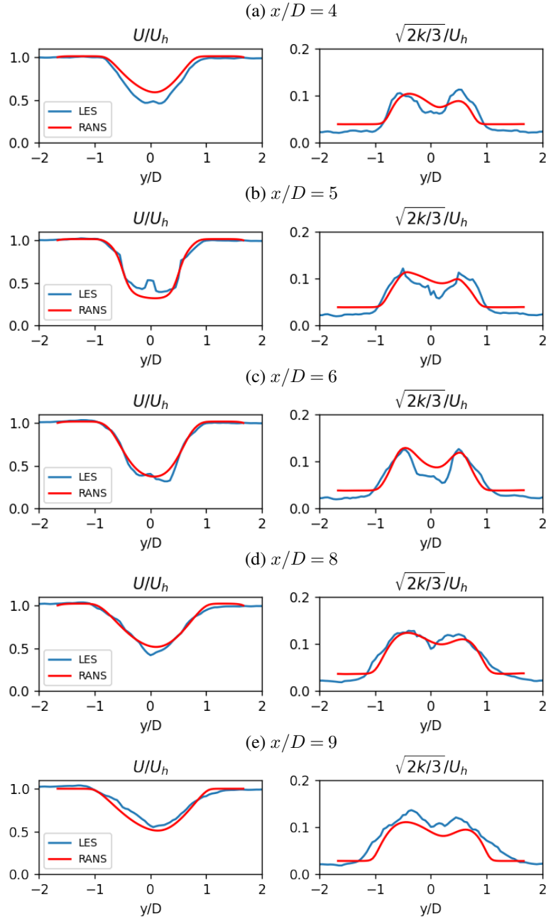
Figure 12. Hub-height profiles of the normalized velocity and TKE for the two-turbine configuration in the Med WS ABL conditions, as computed by the Kynema-SGF LES and SANDWake3D RANS codes. Note that all streamwise distances are measured from the upstream turbine at x/D = 0 , and the second turbine is located at x/D = 5 .
