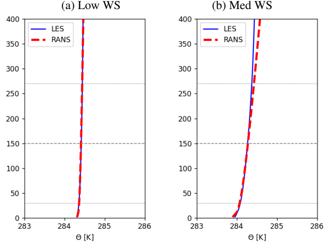
Figure 3. The comparison of the inflow temperature \Theta(z) profiles between RANS and the Kynema-SGF LES computations.
