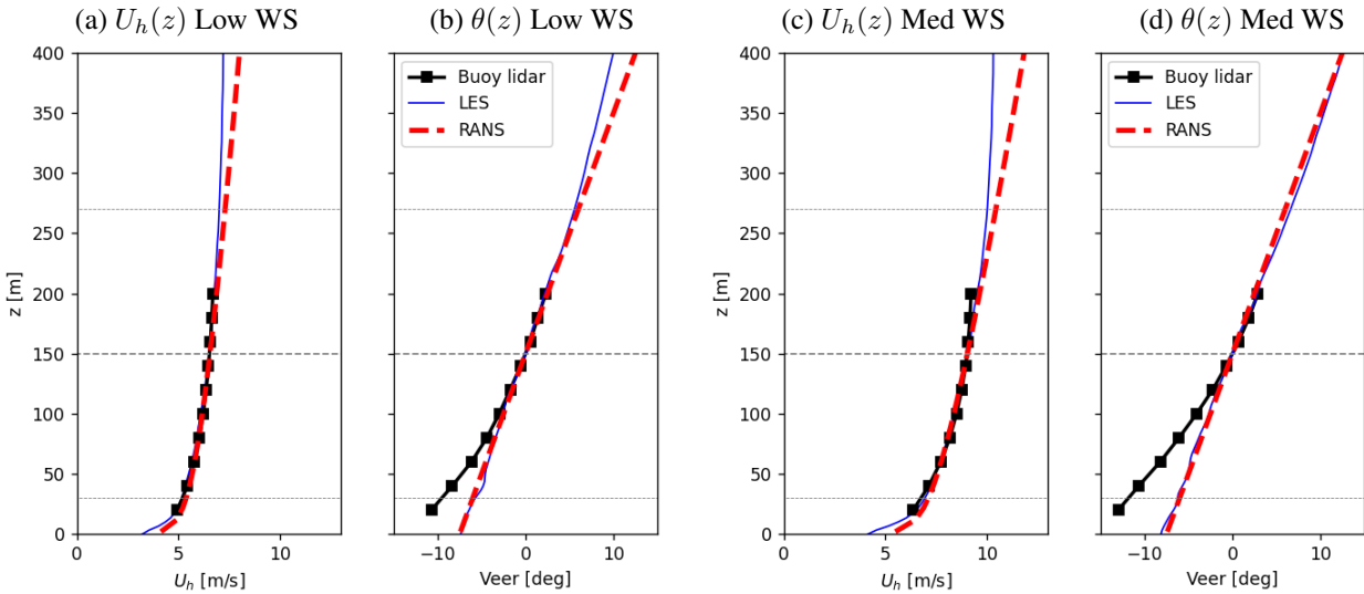
Figure 2. Inflow comparison between the RANS model, Kynema-SGF LES, and the floating buoy lidar data for the horizontal wind speed U_h(z) and veer \theta(z) profiles for the two ABL conditions in table 3.
