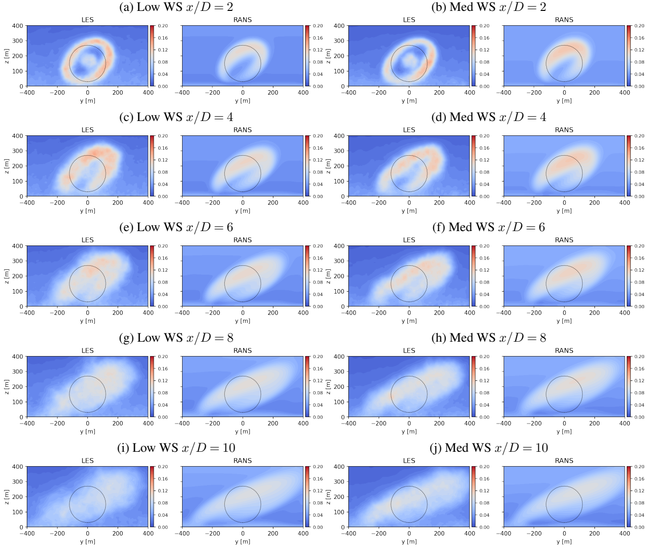
Figure 6. Comparison of the normalized turbulent kinetic energy for the Low and Med WS inflow condition, as computed by Kynema-SGF LES and SANDWake3D RANS methods. Contours of nondimensionalized TKE are plotted at distances x/D = 2, 4, 6, 8, 10 downstream of the turbine. The dashed circle corresponds to the location of the rotor disk of the IEA 15MW reference turbine.
