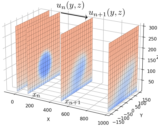
Figure 1. Schematic showing the parabolized RANS solution process by marching planes of the velocity variable u(y, z) downstream through the domain.
