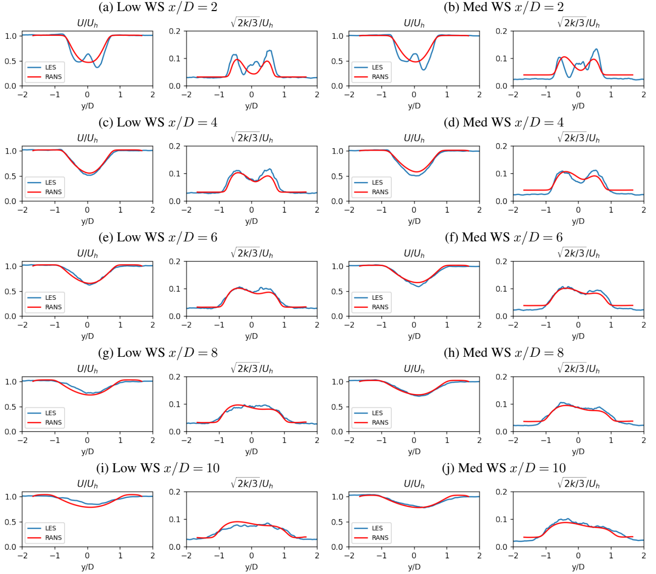
Figure 7. Hub-height profiles of the normalized velocity and normalized TKE \sqrt{2k/3}/U_h for the single turbine wake in the Low WS and Med WS ABL conditions, as computed by the Kynema-SGF LES and SANDWake3D RANS codes.
