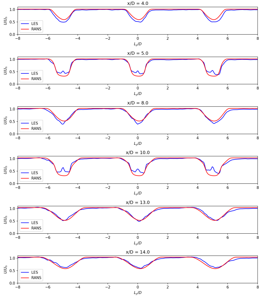
Figure 17. Hub-height profiles of the normalized velocity the 9-turbine wind farm configuration in the Med WS ABL conditions, as computed by the Kynema-SGF LES and SANDWake3D RANS codes. Note that all streamwise distances are measured from the first turbine row at x/D = 0 , the second turbine row is located at x/D = 5 , and the third at x/D = 10 . Note that L_y is the lateral coordinate measured from the center turbine.
