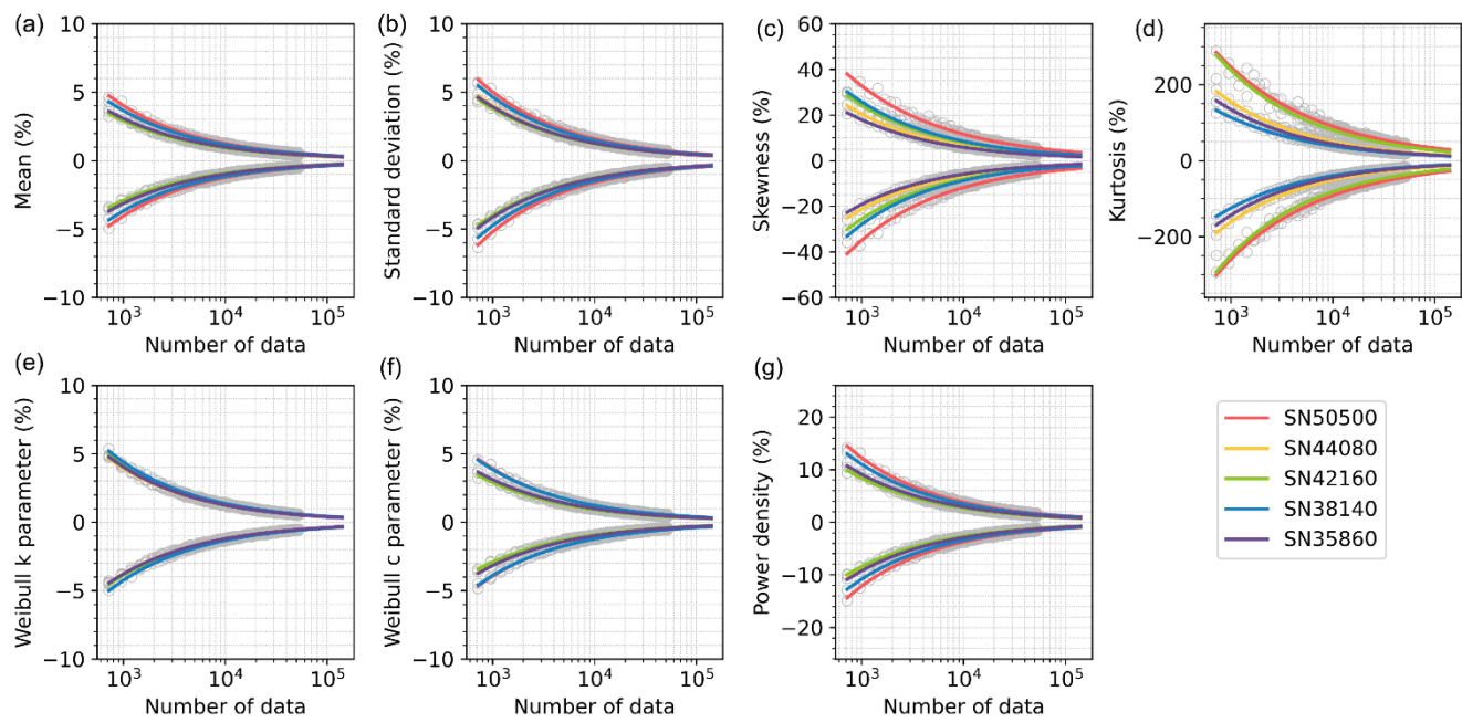
Figure 4: The relationship between the percent error (Y) and sample size (n) (number of hourly observations) across five stations. Curves are fitted for n = 720 \sim 140\,160 , with n = 720 is equivalent in size to 30 days of hourly data and 140 160 equivalent to 16 years. The equations of fits here are shown in Table 3. Grey circles indicate the values used to fit the 90% confidence intervals for the percent error shown.
