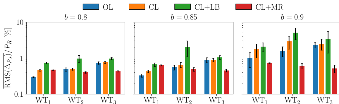
Figure 16. RMS of local power tracking errors for the four APC algorithms and three power-demand power-demand levels b . Static experiment with fixed wind direction \psi = 5.7^\circ , corresponding to 50% rotor overlap. Whiskers indicate 95% confidence intervals.
