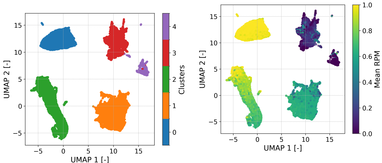
Figure 8. UMAP projection coloured by normalised mean RPM. The smooth gradient indicates that rotor speed is preserved in the embedding.
