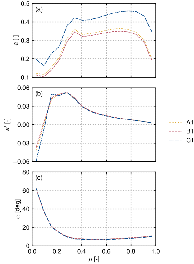
Figure 10. Azimuthally averaged axial induction (a), tangential induction (b), and angle of attack \alpha (c) shown as a function of nondimensional radial position \mu = r/R .
