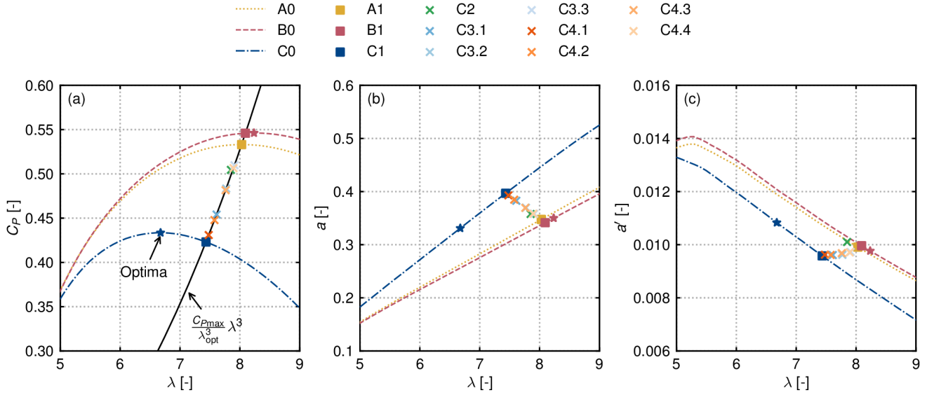
Figure 6. Simulation results for the controlled turbine placed at the different positions: (a) C_P - \lambda curves with control curve in solid black, steady state operational points below rated wind speed marked as crosses and discrete maximum C_P marked by stars, (b) induction curves and operational points with a = 1 - u_R/U_{Ref} where u_R is the kinetic energy mean over the rotor calculated like U_{Ref} in Eq. (10) and (c) tangential induction a' evaluated as azimuthal mean at r = 0.75R .
