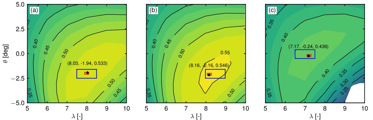
Figure 4. C_P -surfaces obtained in (a) a flat domain A0 , (b) on the foot of the hill B0 and (c) on top of the hill C0 . Black stars indicate the point of optimal power performance. These discrete optima are found by a nested grid search: the outer meshgrid has a spacing of \Delta\lambda = 1 and \Delta\theta = 1 deg, within the blue square the grid spacing is \Delta\lambda = 0.1 and \Delta\theta = 0.1 deg and within the red square the spacing is \Delta\lambda = 0.02 and \Delta\theta = 0.02 deg.
