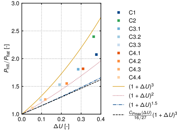
Figure 11. Expected and actual power at the top of the hill for different speed-up factors. The turbines were simulated, including a controller, so the potential maximum power performance would be around one percent higher.
