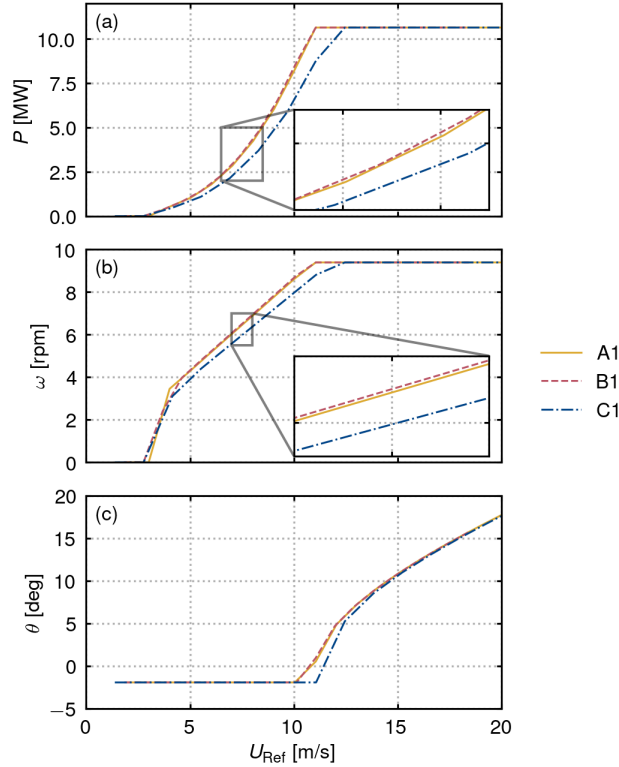
Figure 6. Power curves obtained with the controller in flat terrain ( A1 ), ahead of the hill ( B1 ) and on top of the hill ( C1 ) with the power in (a), the respective rotor speed in (b) and the blade pitch in (c).
