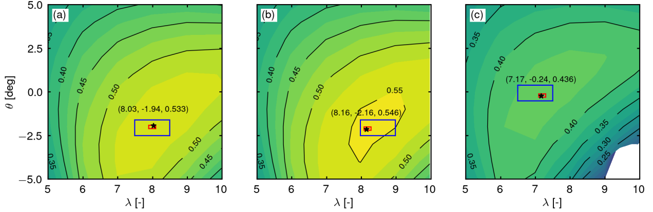
Figure 5. C_P -surfaces obtained in (a) a flat domain A0 , (b) on the foot of the hill B0 and (c) on top of the hill C0 . Black stars indicate the point of optimal power performance. These discrete optima are found by a nested grid search: the outer meshgrid has a spacing of \Delta\lambda = 1 and \Delta\theta = 1 deg, within the blue square the grid spacing is \Delta\lambda = 0.1 and \Delta\theta = 0.1 deg and within the red square the spacing is \Delta\lambda = 0.02 and \Delta\theta = 0.02 deg.
