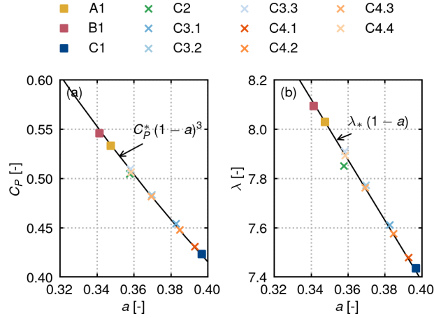
Figure 10. Power coefficient in (a) and tip-speed ratio in (b) as a function of the induction in flat terrain, ahead of the hill and on top of it together with Eq. (21) and Eq. (23) using C_P^* = 1.92 and \lambda_* = 12.31 .
