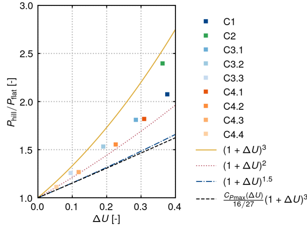
Figure 12. Expected and actual power at the top of the hill for different speed-up factors. The turbines were simulated, including a controller, so the potential maximum power performance would be around one percent higher.
