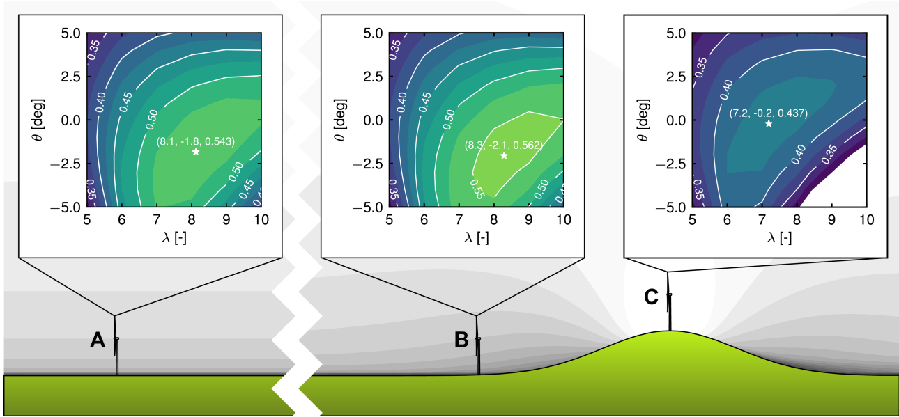
Figure 2. C_P surfaces obtained in a flat domain ( A0 , left), on the foot of the hill ( B0 , center) and on top of the hill ( C0 , right). White stars indicate the point of optimal power performance. Iso-curves of the undisturbed flow velocity magnitude in the graphic illustrate regions of speed-up in the vicinity of the hill.
