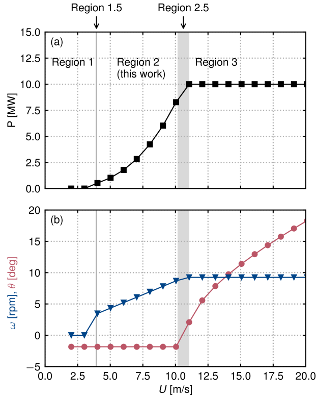
Figure 1. An example of a power curve of a wind turbine with the different control regions labeled: (a) Power and (b) rotor speed \omega and blade pitch \theta .
