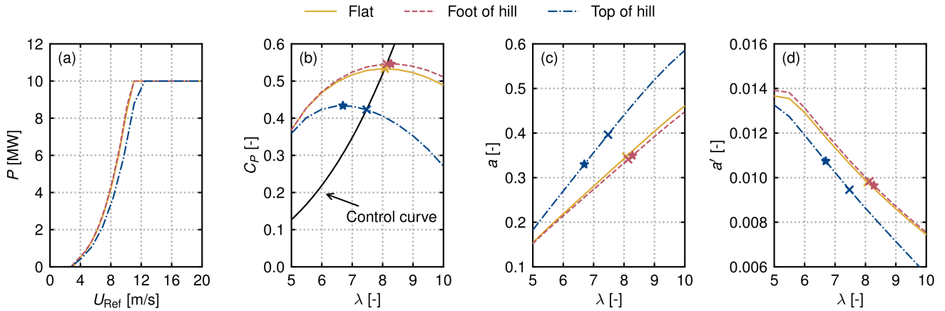
Figure 3. Simulation results for the controlled turbine placed at the three different positions ( A1 , B1 , C1 ): (a) Power curves, (b) C_P - \lambda curves with control curve in solid black, steady state operational points below rated wind speed marked as crosses and maximum C_P marked by stars, (c) induction curves and operational points with a = 1 - u_R/U_{Ref} where u_R is the kinetic energy mean over the rotor calculated like U_{Ref} in Eq. (9) and (d) tangential induction a' = u_{R,t}/(\omega r) evaluated as azimuthal mean at r = 0.75R .
