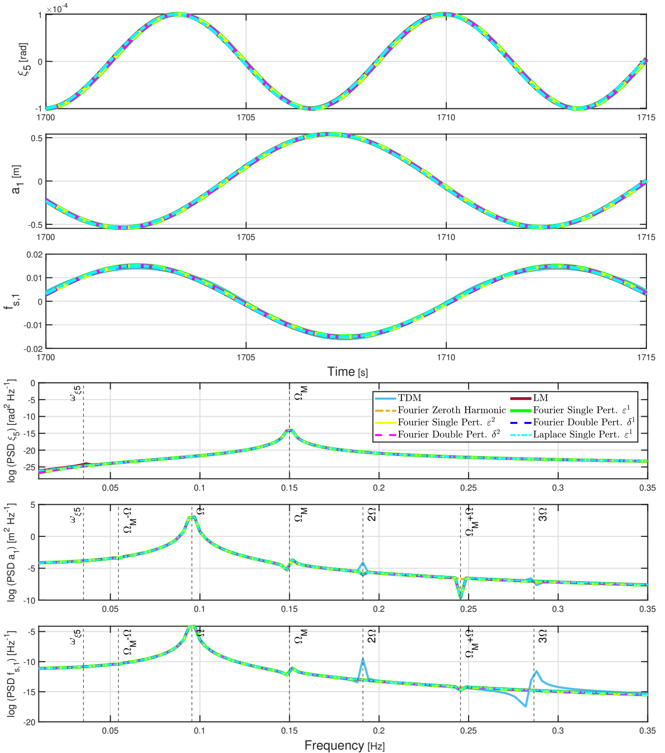
Figure 4. Time series and PSD plots for load case B with the operational point of V_0 = 8 \text{ m s}^{-1} and \Omega = 0.6 \text{ rad s}^{-1} .
