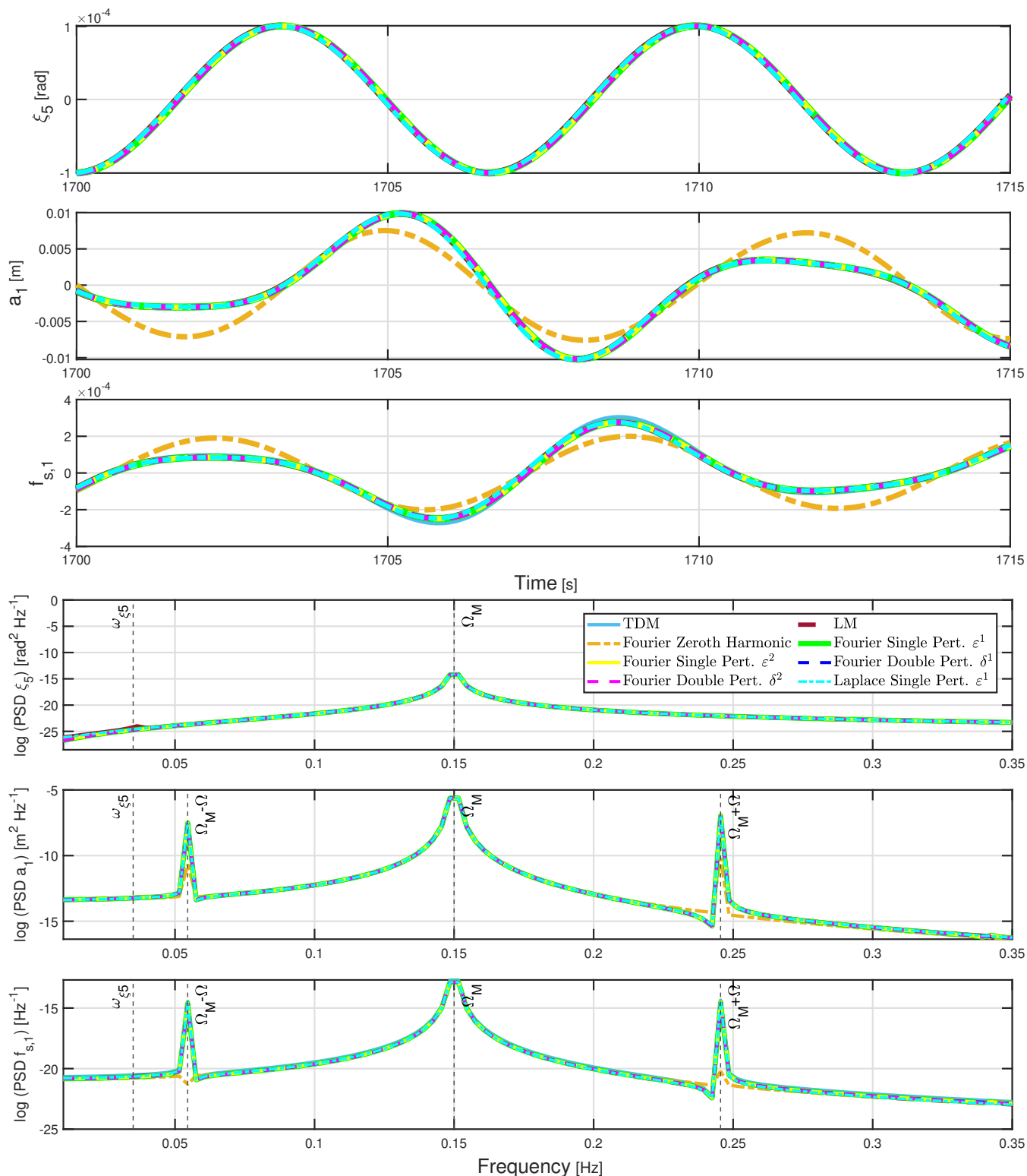
Figure 3. Time series and PSD plots for load case A with the operational point of V_0 = 8 \text{ m s}^{-1} and \Omega = 0.6 \text{ rad s}^{-1} .
