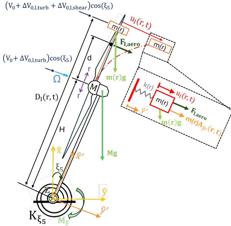
Figure 1. Floating wind turbine model where blade properties and parameters vary in the radial direction r and with blade index l . This includes the blade deflection u_l(r, t) and the distance of a blade element mass m(r) from the floater base being D_l(r, t) .
