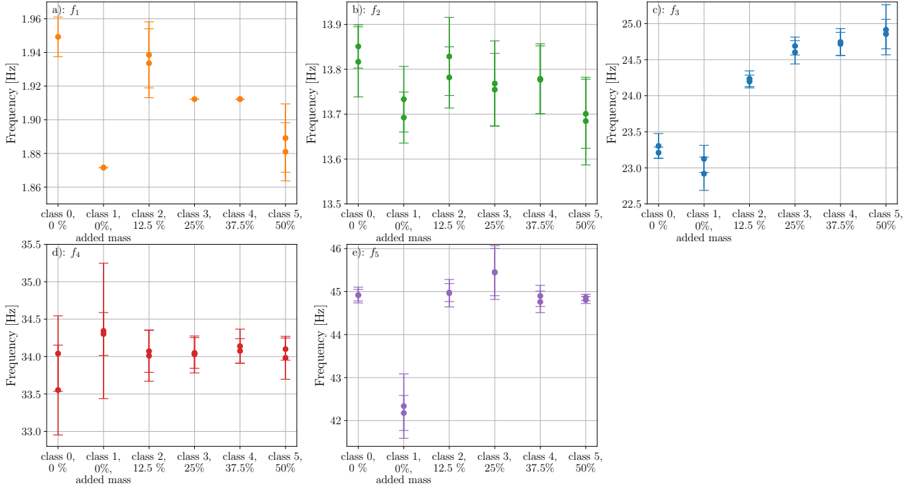
Figure 12. Evolution of the mean values (circular markers) and standard deviations (error bars) of the first five eigenfrequencies f_i , determined with AFDD and clustering , plotted over the damage classes. The exact values of f_i for each damage class are given in Table A4. Eigenmode \phi_1 could not be detected in experiment 6 and 63 which correspond to damage class 0 and 3. Thus for f_1 , there is only one value presented in damage classes 0 and 3.
