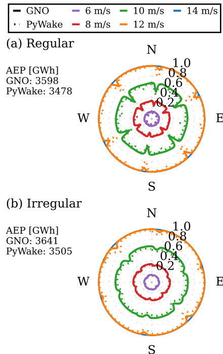
Figure 10. Normalized power production at different wind speeds and TI=5\% I_0=5\% , illustrated as wind roses-power roses for the IEA Wind 740-10-MW reference wind farm (Kainz et al., 2024). (a) Regular layout pre-optimization and (b) Irregular optimized layout.
