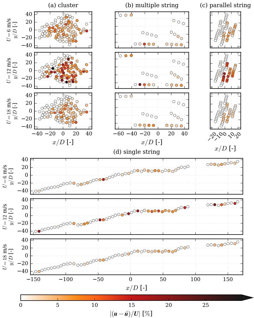
Figure E1. Maximum absolute errors at each wind turbine, for each wind speed in U = [6, 12, 18]^T ms -1 and I_0 = 5\%
