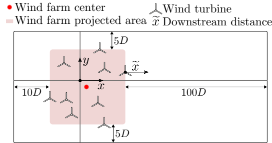
Figure 3. Adaptive computational grid for generating flow maps with PyWake. 195
