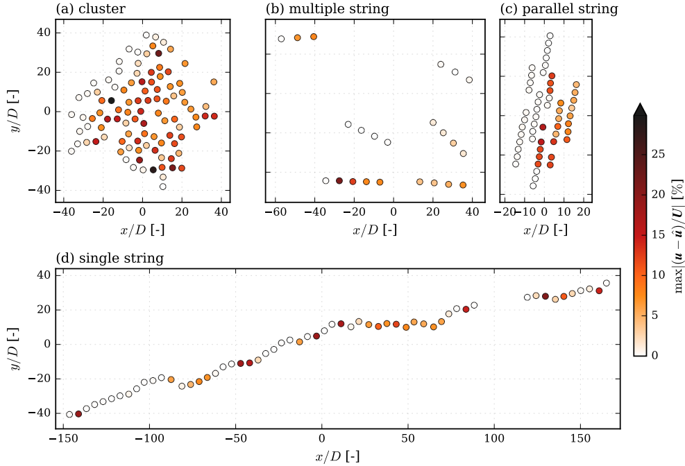
Figure 9. Maximum absolute errors at each wind turbine, for \mathbf{U} = [6, 12, 18]^\top \text{ ms}^{-1} and I_0 = 5\%
