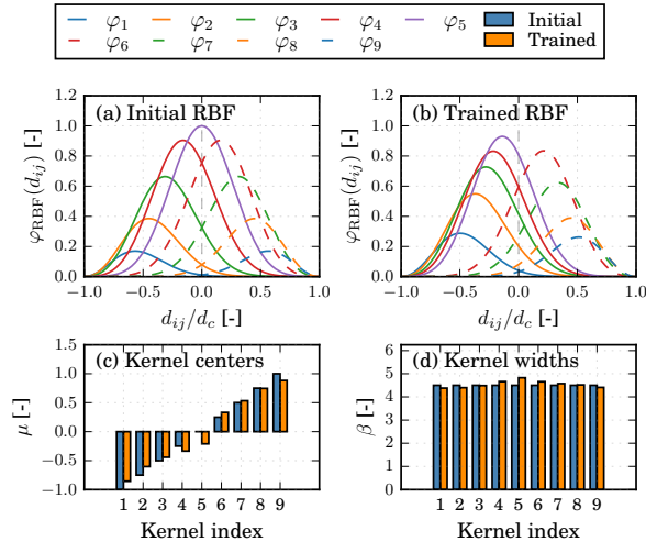
Figure 13. RBF kernels (a) before and (b) after training, with (c) kernel centers \mu and (d) kernel widths \beta shown before and after training.
