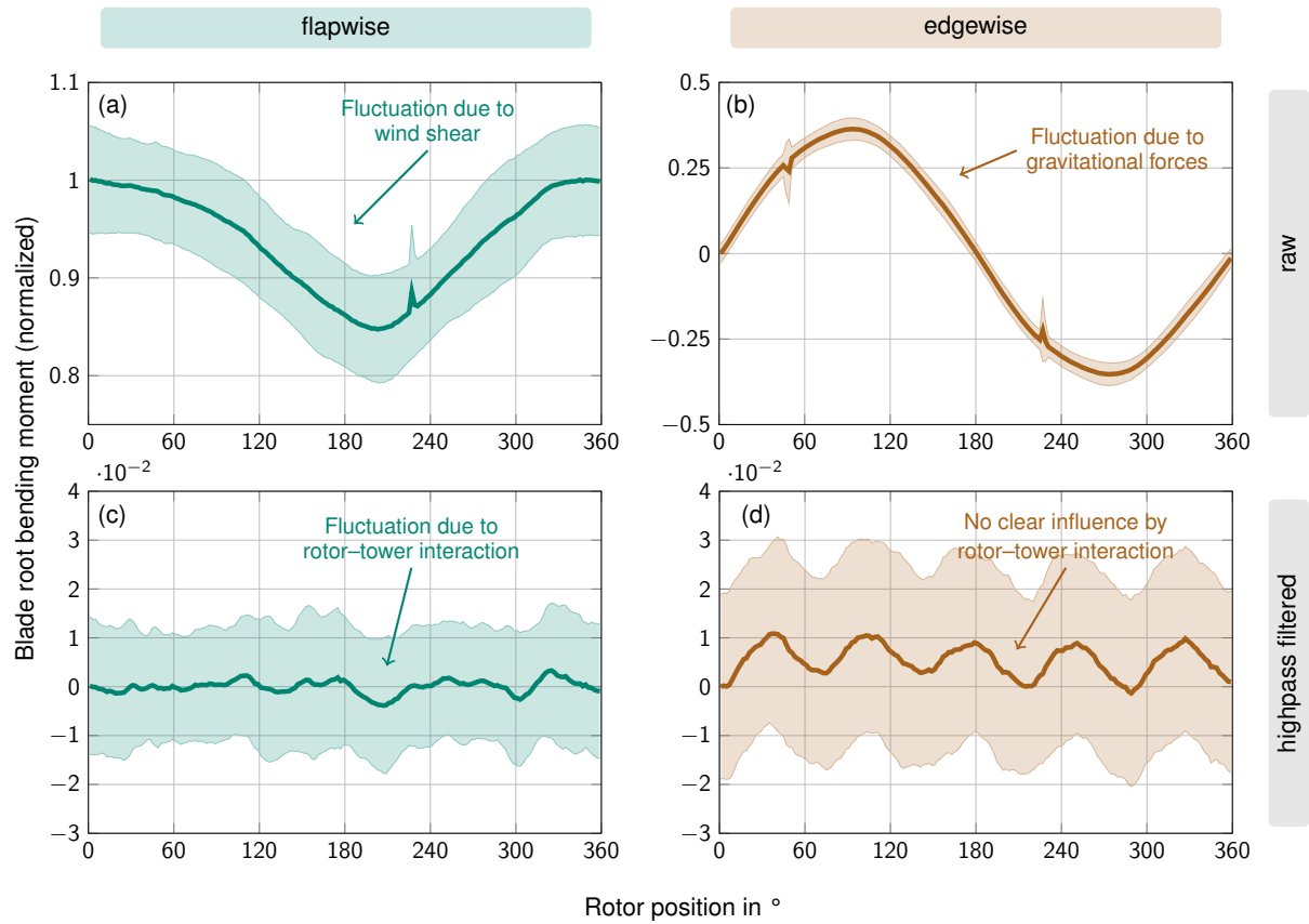
Figure 20. Flapwise (left column) and edgewise (right column) root bending moments of one rotor blade as a function of rotor position for the operating point U_\infty = 11.12 \text{ m/s} ( U_\infty = 11.12 \text{ ms}^{-1} ) (Table 1). The top row shows the raw signal, while the bottom row shows the high-pass filtered signal. For confidentiality reasons, the data were normalized to the maximum flapwise bending moment. The shaded areas indicate the standard deviation of the 10-minute average.
