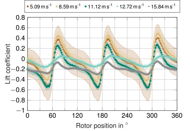
Figure 11. Lift coefficient of the tower as a function of rotor position. The different curves correspond to different wind speeds. The shaded areas indicate the measurement uncertainty in the 95 % confidence interval. The curves have been corrected for inconsistent rotor position timestamps and aligned so that the first pressure minimum appears at 60^\circ .
