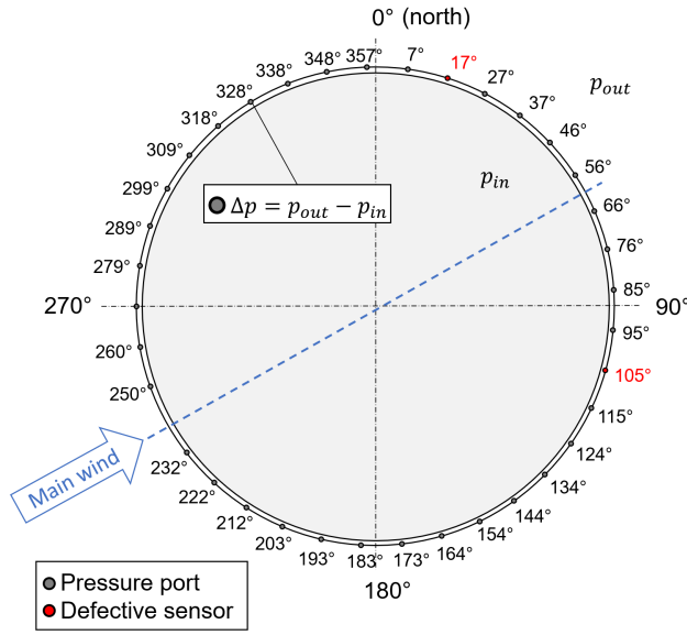
Figure 3. Distribution of pressure ports on the belt in the earth-fixed coordinate system (0° facing north). The differential pressure is measured between the tower surface ( p_{out} ) and the inside of the tower ( p_{in} ). Two defective sensors (marked in red) were excluded from the analysis.
