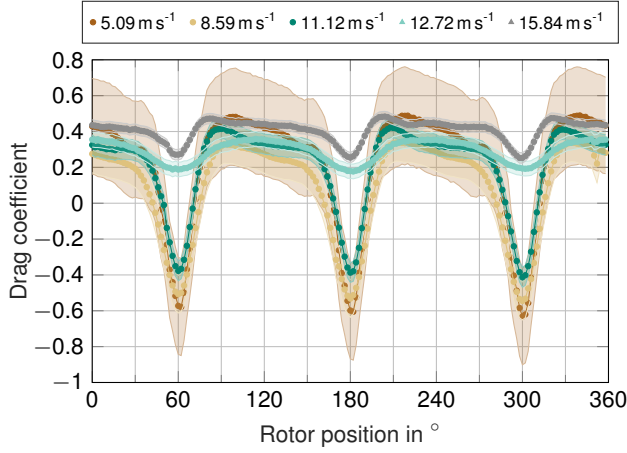
Figure 10. Drag coefficient of the tower as a function of rotor position. The different curves correspond to different wind speeds. The shaded areas indicate the measurement uncertainty in the 95 % confidence interval. The curves have been corrected for inconsistent rotor position timestamps and aligned so that the first pressure minimum appears at 60^\circ .
