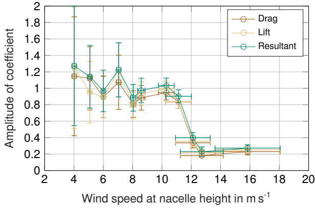
Figure 14. Maximum amplitude of the resultant force coefficient (corresponding to the maximum diameter of the curves in Fig. 12) as a function of the free stream velocity. Results are shown for all operating points listed in Table 1. The vertical error bars indicate the measurement uncertainty in the 95 % confidence interval. The horizontal error bars represent the standard deviation of the 10-minute average wind velocity.
