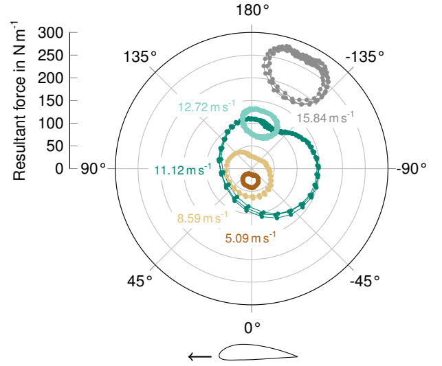
Figure 13. Mean resultant force plotted against the corresponding angle relative to the free stream direction (see Fig. 4 for angle definition). Different curves correspond to different wind speeds.
