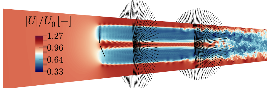
Figure 4. Two radial probes superimposed on a longitudinal domain slice. The probes are shown as black dots. The slice was colored by the instantaneous streamwise velocity contours at t/T_p = 4 for the SuLS case, where T_p = 1/f_p .
