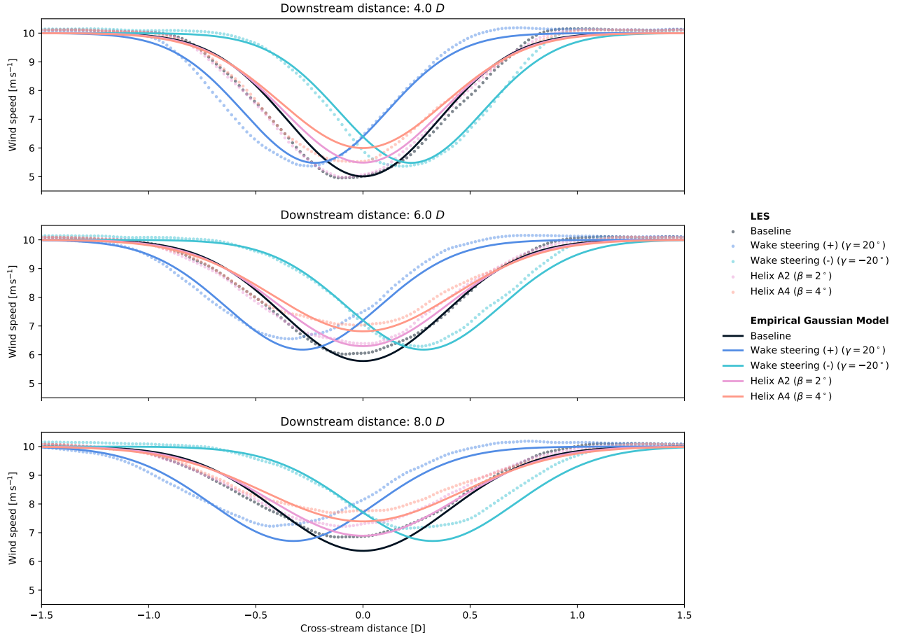
Figure A2. Wind speed deficit modeled using the Empirical Gaussian model and LES data, considering no control (“baseline”), wake steering, and helix control, shown for down-stream distances of 4D , 6D , and 8D . The plots refer to one-turbine simulations.
