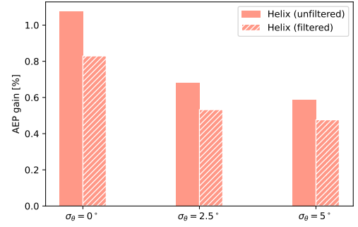
(b) AEP gains comparison between filtered and unfiltered helix control setpoints.
