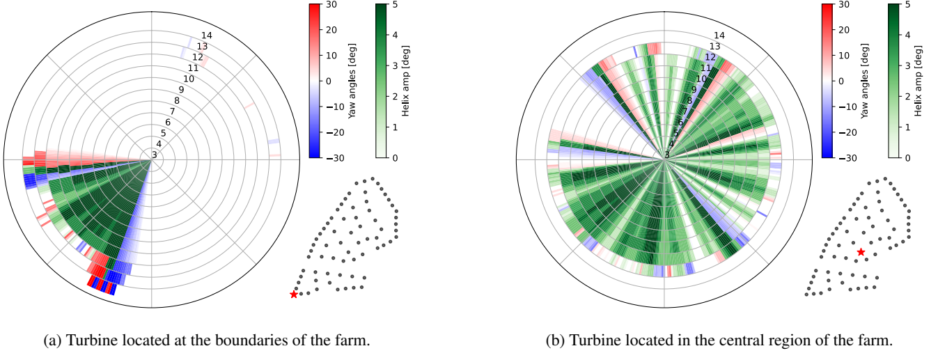
Figure 10. Control rose for the combined strategy of two different turbines. The exact position of the turbines are is highlighted in the wind farm layout included in each subplot. Each subplot includes the values of the control variables present present in the LUT for each wind speed and direction, obtained for with a wind direction uncertainty of \sigma_\theta = 2.5^\circ .
