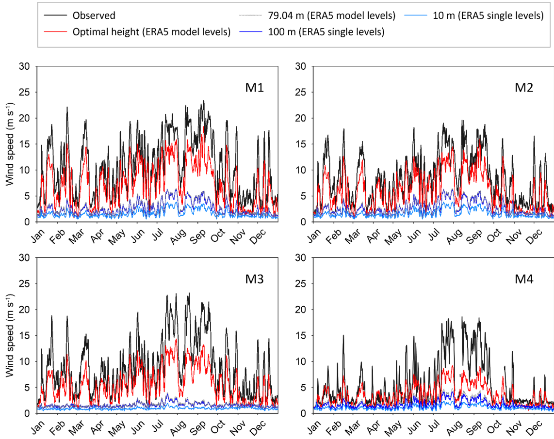
Figure 63: Wind speed time series for the observations and ERA5 data in 2024. The times series shows the 24 h running average instead of the hourly time series for visualization proposes. Note that at M1, M2 and M3, the wind speed series at 100 m (ERA5 single level) and 79.04 m (ERA5 model level) overlap.
