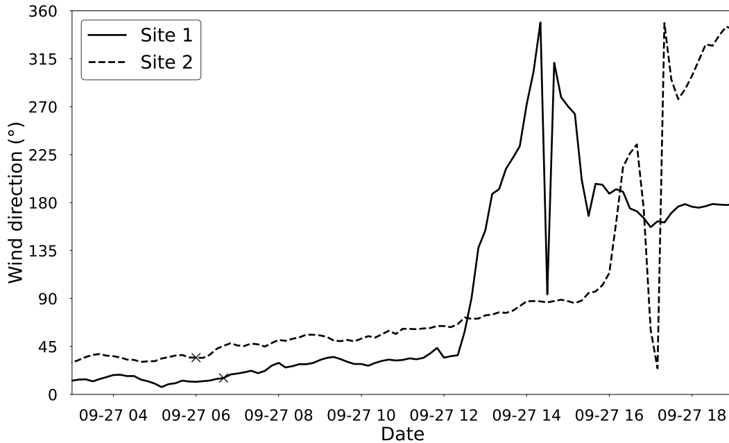
Figure 18. Time series of wind direction during TC Megi at sites 1 and 2. The crosses correspond to the instants of maximum wind speed measured on site the measurement sites .
