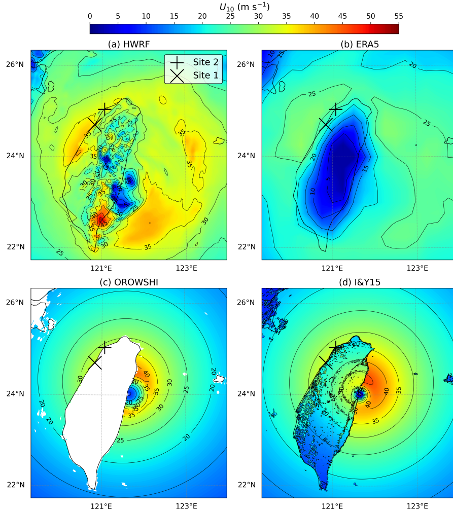
Figure 19. Comparison of V_m (2D) and Bias Error from IBTrACS and predicted by the models for TC Megi surface wind field on 27 September at 6 A.M. GMT. Model IBTrACS predicted by HWRf (a), ERA5 (b), OROWSHI I&wind model (c) and I&Y15 ERA5-HWRf V_m/BE ( m \cdot s^{-1} wind model) (d) 47.8 46.9 / -0.9 46.0 / -1.8 28.9 / -18.9 52.3 / 4.5.
