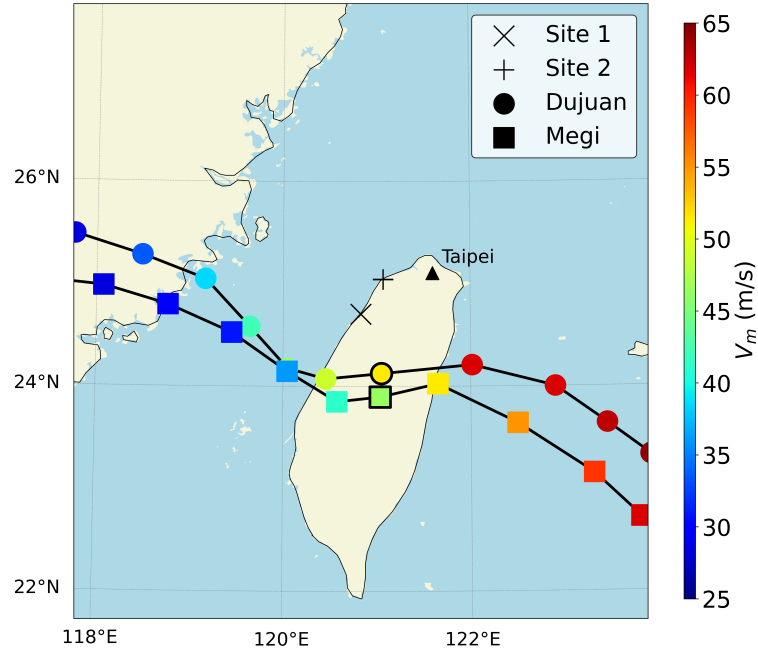
Figure 5. Measurement sites impacted by Typhoon Dujuan (sites: \times & + , track: \bullet ) (2015) & Megi (site: + , track: \blacksquare ) (2016).
