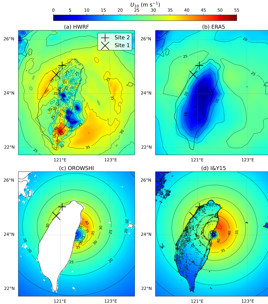
Figure 19. TC Megi surface wind field on 27 September at 6 A.M. GMT predicted by HWRf (a), ERA5 (b), OROWSHI wind model (c) and I&Y15 wind model (d).
