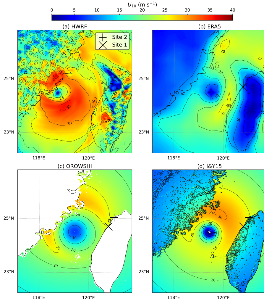
Figure 20. TC Megi surface wind field on 27 September at 6 P.M. GMT predicted by HWRP (a), ERA5 (b), OROWSHI wind model (c) and I&Y15 wind model (d).
