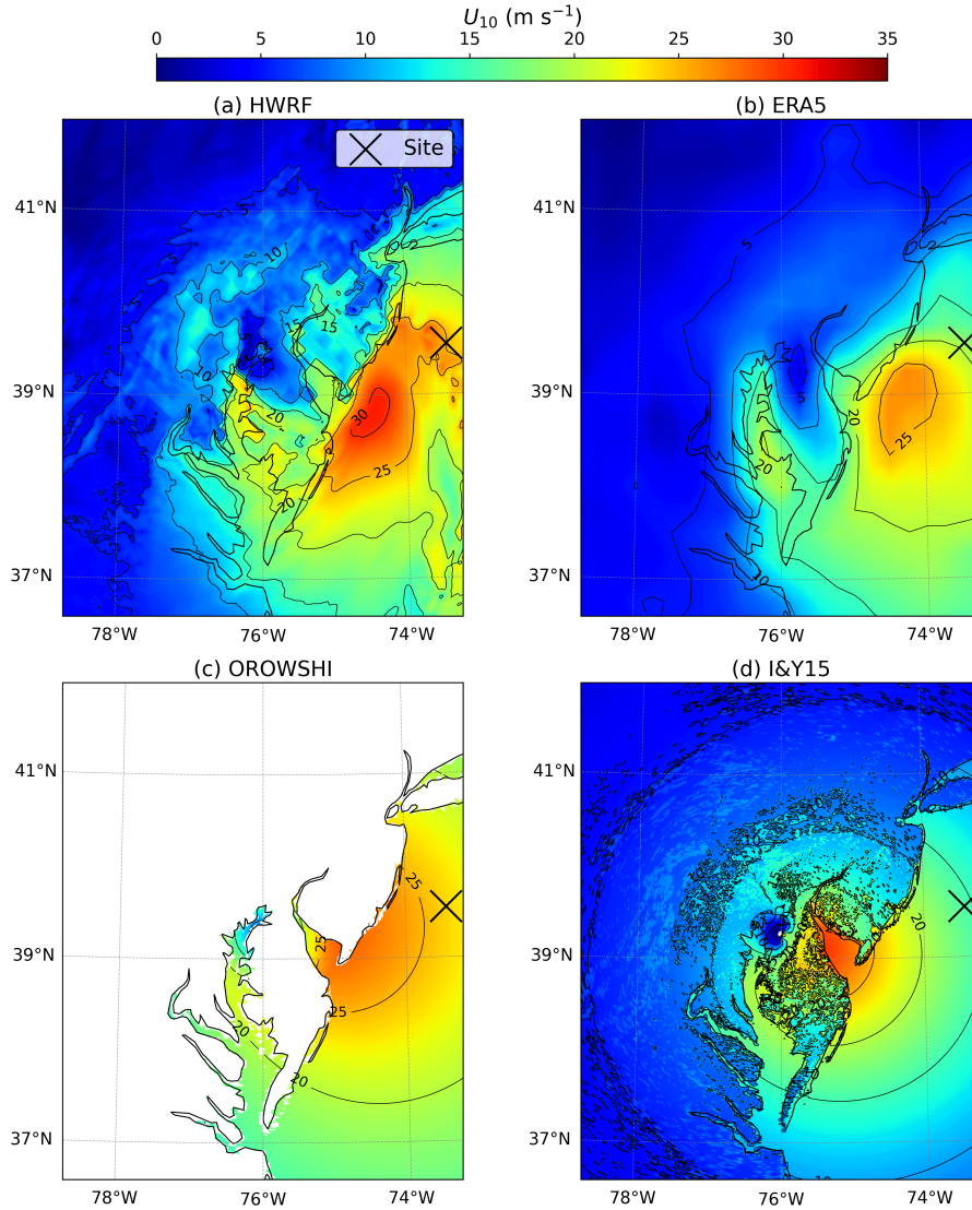
Figure 14. TC Isaias surface wind field on 8 August at 3 P.M. GMT predicted by HWRP (a), ERA5 (b), OROWSHI wind model (c) and I&Y15 wind model (d).
