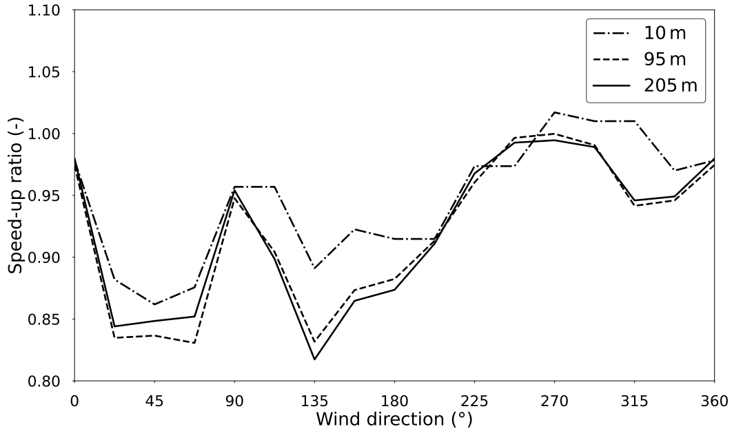
Figure 3. Variation of the speed-up ratio with wind direction at 10 m, 95 m and 205 m above the mean sea level, computed using the MASCOT software.
