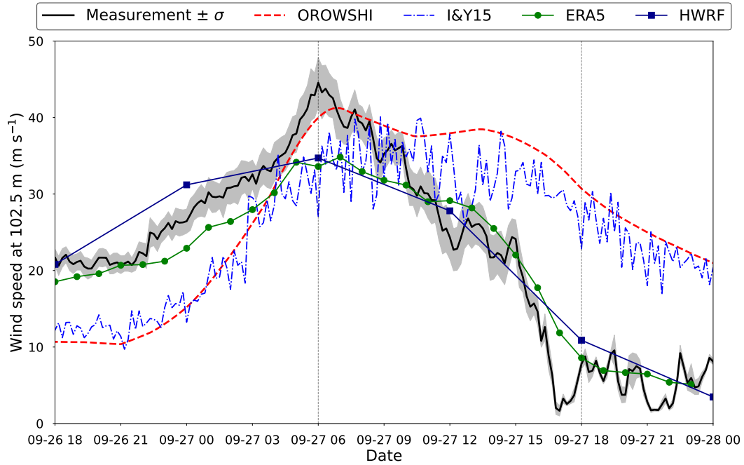
Figure 17. Time series of observed and predicted winds of TC Megi at 102.5 m (site 2). The vertical dashed lines correspond to the instants at which the surface wind field is assessed.
