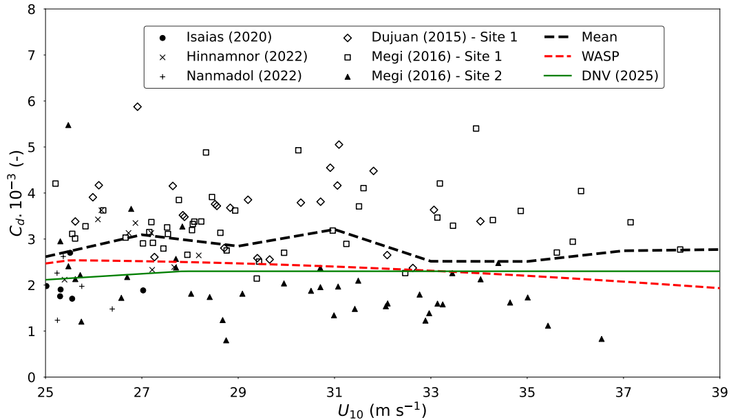
Figure 6. Drag coefficient as a function of surface wind U_{10} . Comparison between WASP, DNV (2025) and the measurements. The black dashed line corresponds to the mean measured value for bins of 2 \text{ m s}^{-1} .
