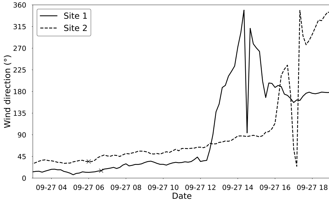
Figure 18. Time series of wind direction during TC Megi at sites 1 and 2. The crosses correspond to the instants of maximum wind speed measured on the measurement sites.
