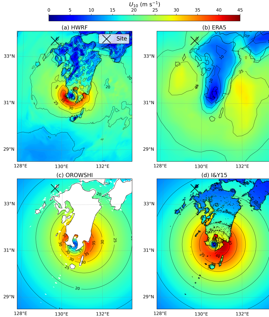
Figure 11. TC Nanmadol surface wind field on 18 September at 9 A.M. GMT predicted by HWRF (a), ERA5 (b), OROWSHI wind model (c) and I&Y15 wind model (d).
