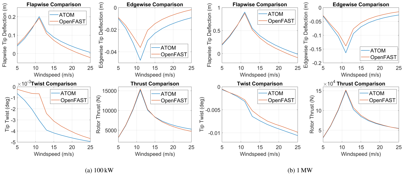
Figure 13. Structural deformations at the blade tip for (a) 100kW and (b) 1 MW blade designs, compared between ATOM and OpenFAST. Rotor thrust is included to demonstrate the proximity in forces as opposed to the discrepancies in deflection, which suggests that the differing deflections are due to differences in the structural models.
