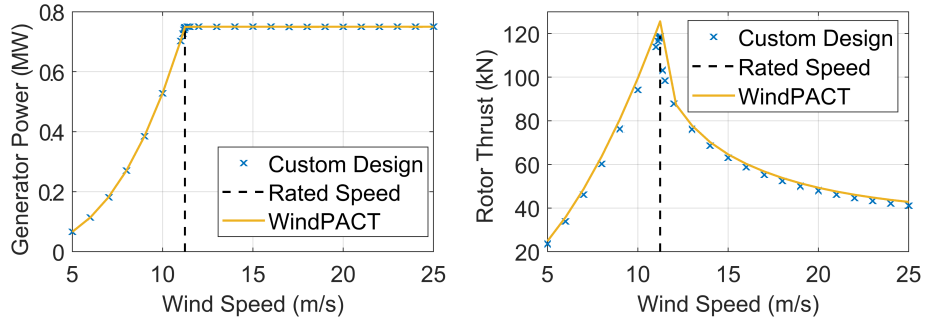
(a) Rotor power and thrust comparison
