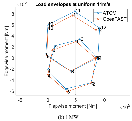
Figure A3. Load envelopes calculated at the blade root for the (a) 100 kW and (b) 1 MW reference blades in 11 m/s (near-rated) uniform wind conditions. To remove transient effects, the first 3 seconds of the 30 second simulation are omitted.
