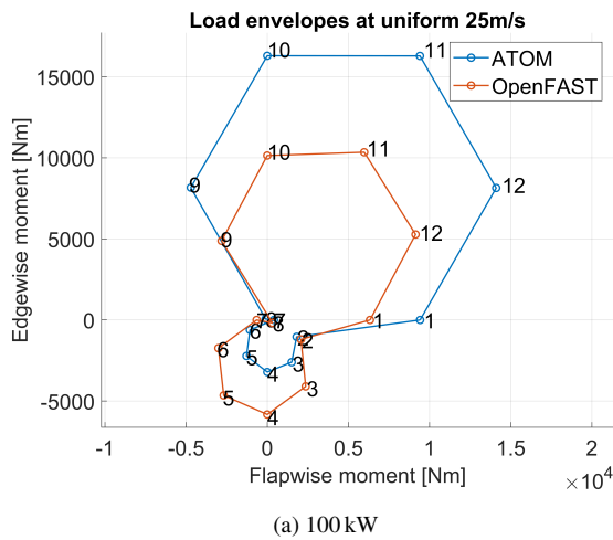
Figure A4. Load envelopes calculated at the blade root for the (a) 100 kW and (b) 1 MW reference blades in 25 m/s (cut-out) uniform wind conditions. To remove transient effects, the first 3 seconds of the 30 second simulation are omitted.
