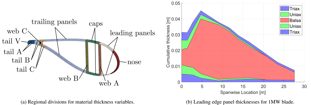
Figure 4. Depiction of material thickness DVs, along with an example of the leading panel thicknesses from the 1 MW design. The thickness of each layer in each region is set as an active design variable. (a) is reproduced with permission from (Bak et al., 2013).
