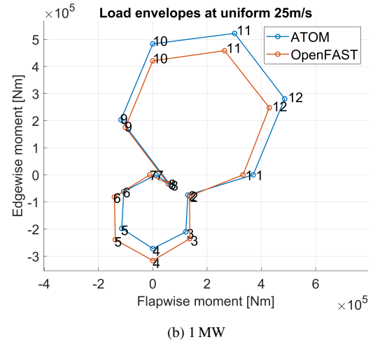
Figure A4. Load envelopes calculated at the blade root for the (a) 100 kW and (b) 1 MW reference blades in 25 m/s (cut-out) uniform wind conditions. To remove transient effects, the first 3 seconds of the 30 second simulation are omitted.
