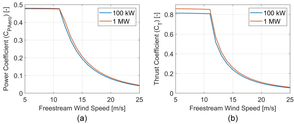
Figure 10. Dimensionless (a) aerodynamic power (not including electrical or drivetrain losses) and (b) thrust coefficients of 100 kW and 1 MW custom blade designs, as a function of freestream wind velocity.
