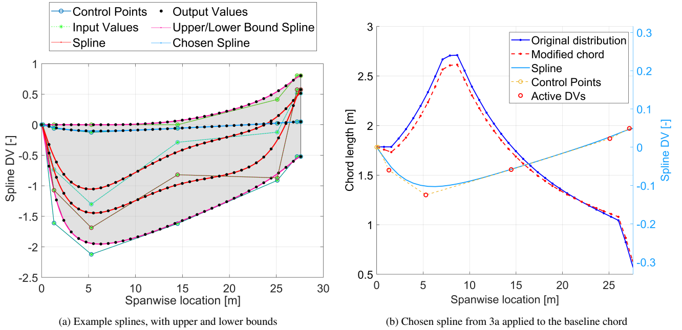
Figure 3. Illustration of "baseline plus spline" design variable adjustment process as applied to the chord distribution of a 1 MW blade design. (a) displays the range of spline curves that can be generated based on the design variable bounds (shaded in grey), and (b) shows the baseline and modified chord distributions following the implementation of the blue spline curve highlighted in (a).
