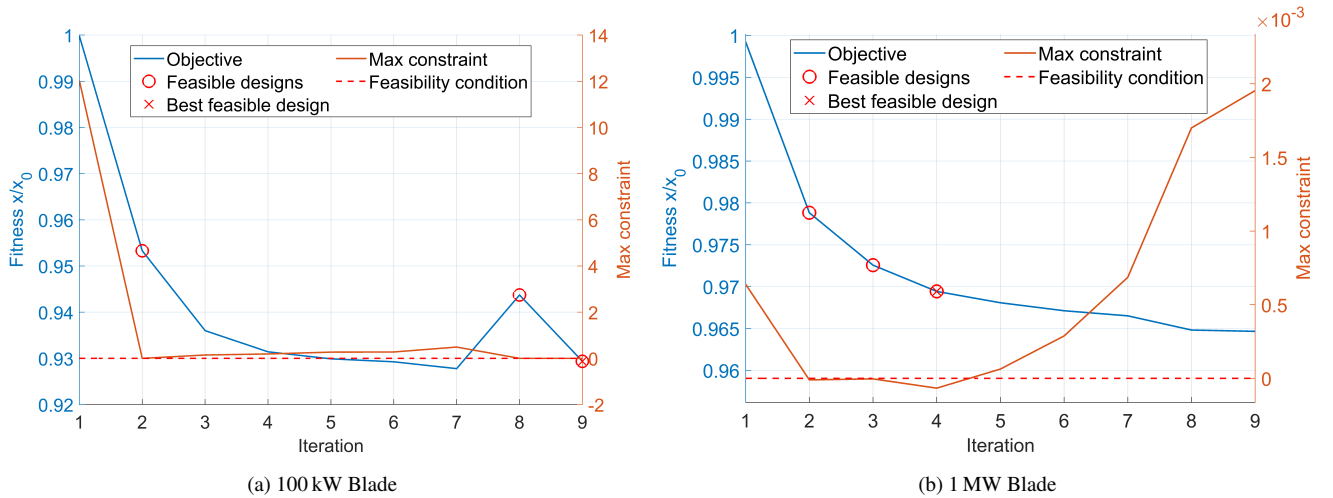
Figure 8. Optimisation histories for 100 kW and 1 MW blades. For a design to be feasible, the maximum constraint must be below zero — a threshold which is marked by a dotted red line. The feasible designs are marked on the blue objective curve with a red circle, and the feasible design with the lowest corresponding objective value is marked with a red cross.
