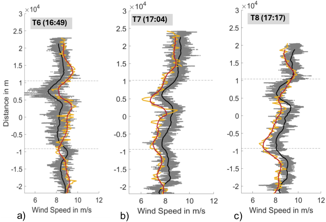
Figure 3. Comparison of airborne wind measurements of D-IBUF at hub height (running mean, black) showing substantial small-scale variability (gray shading) with collocated SAR-derived wind speed (red) and variability (yellow) on 11 September 2021. The SAR wind speed was extrapolated from an altitude of 10 m to hub height using stability information obtained from the flight. The gaps in the SAR-derived data are caused by quality filtering of unrealistic SAR wind speed values due to turbine-related SAR artifacts close to the wind farm Amrumbank West. Panels (a), (b), and (c) correspond to different sampling times (in UTC) and transects called T6, T7 and T8 of the flight data. One flight leg of around 45 km length requires a flight time of around 12 min.
